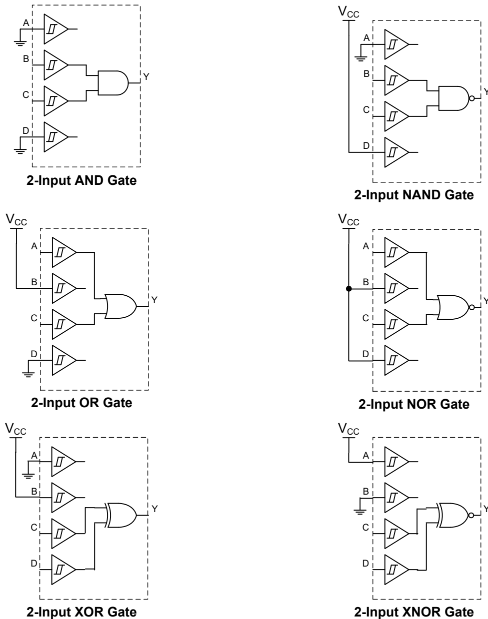
Figure 7-3. Logic Configurations
