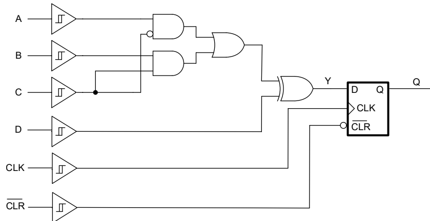
Logic Diagram (Positive Logic)
