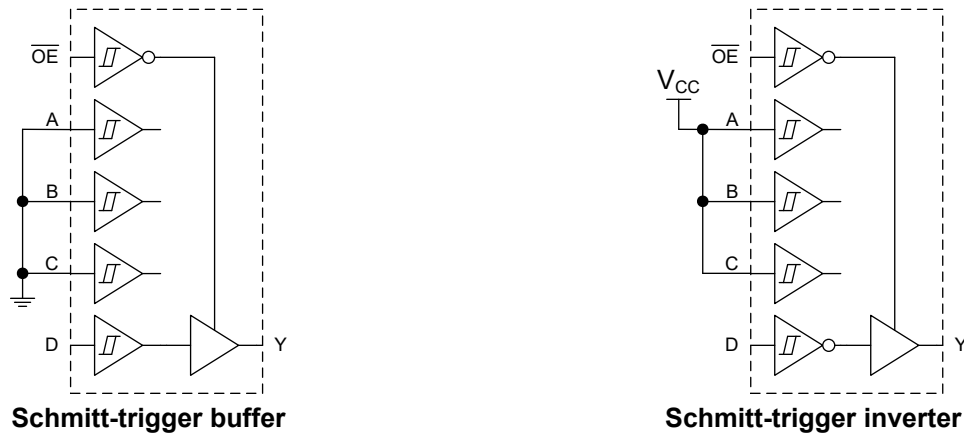
Figure 7-1. Logic Configurations
