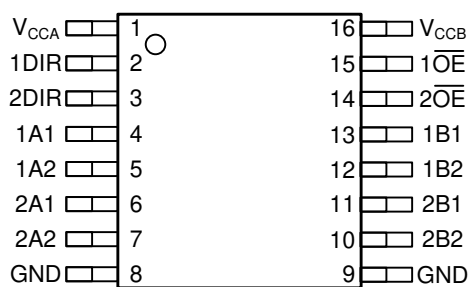
Figure 4-2. PW Package, 16-Pin TSSOP (Top View)
