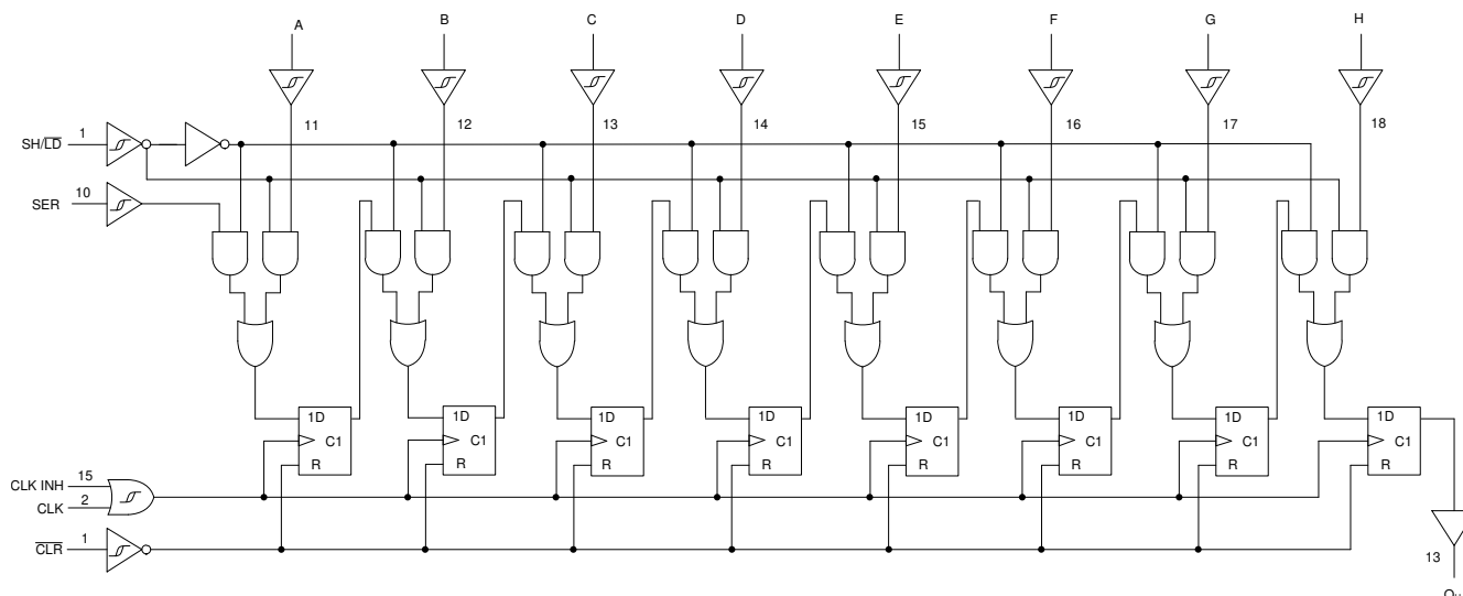
Figure 8-1. Logic Diagram (Positive Logic) for SN74HCS166-Q1
