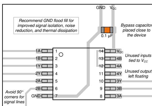
Figure 8-3. Example Layout for the SN74HCS266
