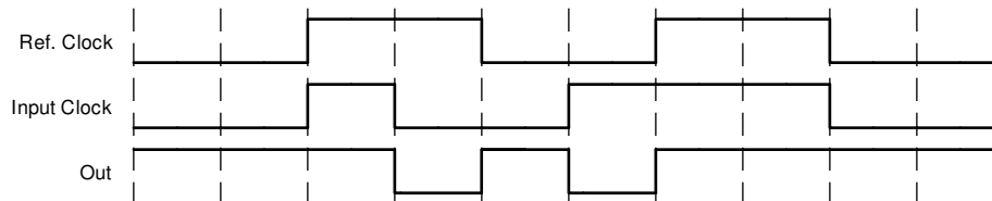
Figure 8-2. Application Timing Diagram
