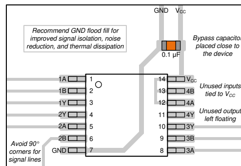
Figure 8-3. Example Layout for the SN74HCS7266-Q1
