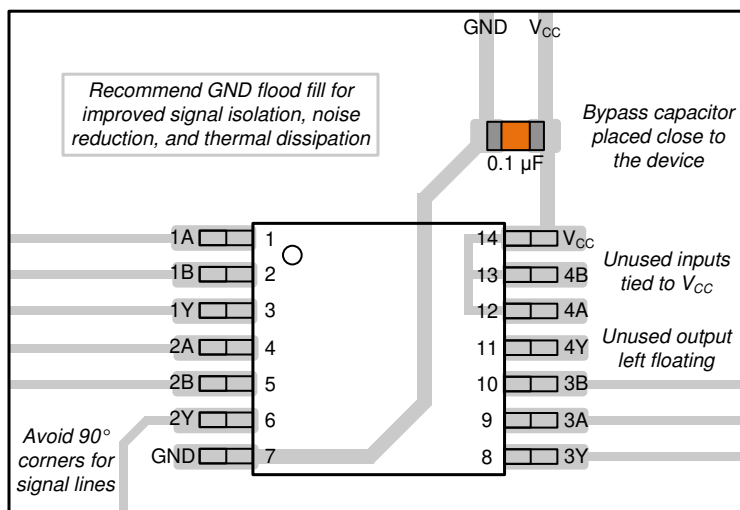
Figure 12-1. Example Layout for the SN74LV4T00-Q1
