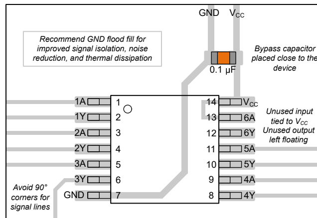
Figure 8-3. Example Layout for the SN74LV6T06-EP
