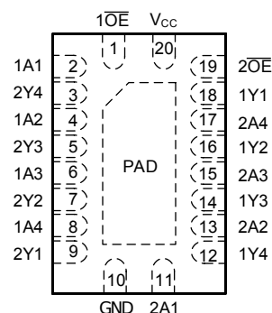
Figure 4-2. SN74LV8T240-Q1 RKS Package; 20-Pin TSSOP (Top View)
