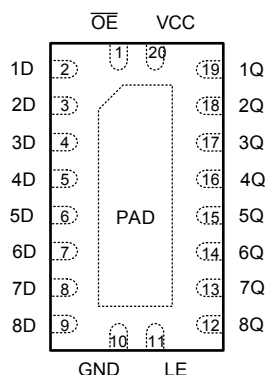
Figure 4-1. SN74LV8T573 RKS Package (Top View)
