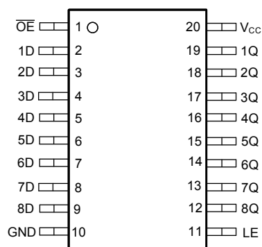
Figure 4-2. SN74LV8T573 PW, DGS Package (Top View)
