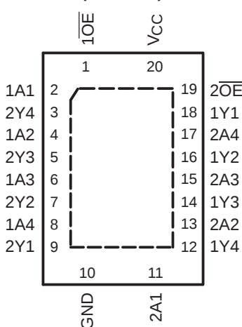
SN74LVCH244A . . . RGY PACKAGE (TOP VIEW)
