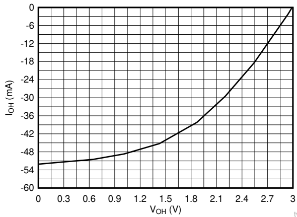
Figure 8-2. LVC family typical output voltage in the high state
