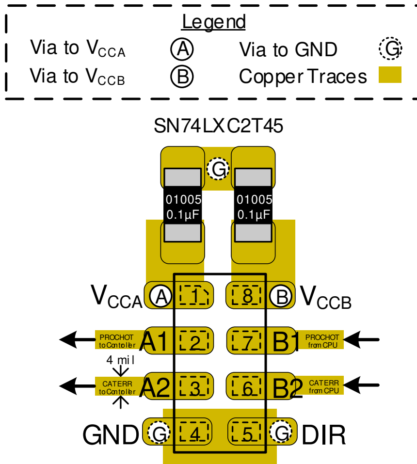
Figure 19-1. Layout Example—SN74LXC2T45DTT
