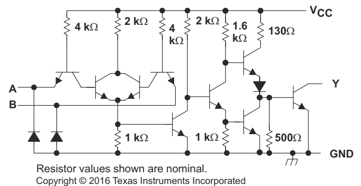
Figure 8-12. SNx5454B Schematic (Each Driver)
