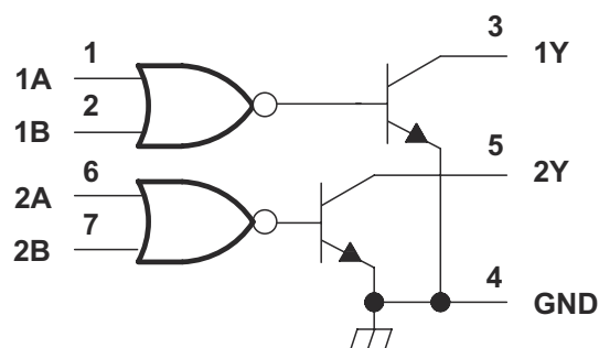
Figure 8-2. SNx5452B Logic Diagram (Positive Logic)
