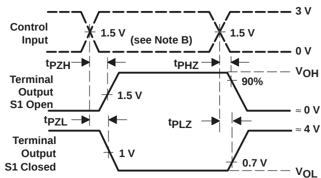
VOLTAGE WAVEFORMS
