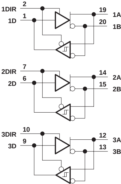
logic diagram (positive logic)
