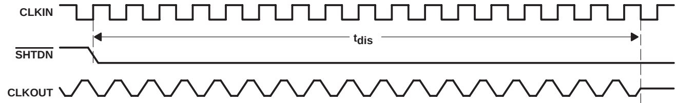
Figure 10. Disable Time
