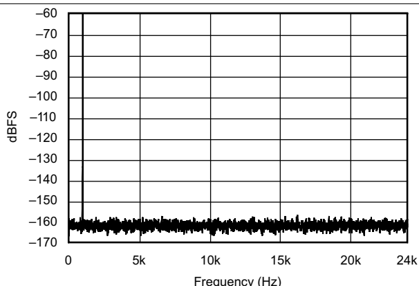
Figure 4. FFT With 1 kHz Input Tone at -60 dBFS (32 kHz:48 kHz)
