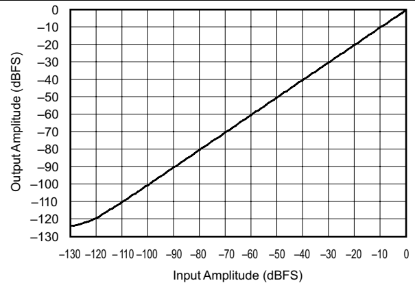
Figure 54. Linearity With f_{IN} = 200\text{ Hz} (44.1 kHz:192 kHz)
