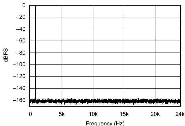
Figure 5. FFT With 1 kHz Input Tone at 0 dBFS (44.1 kHz:48 kHz)
