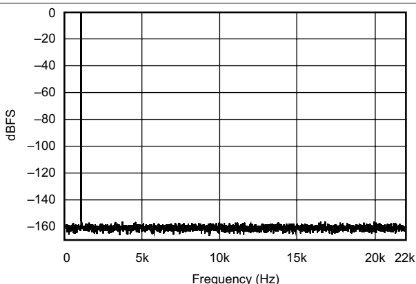
Figure 27. FFT With 1 kHz Input Tone at 0 dBFS (192 kHz:44.1 kHz)
