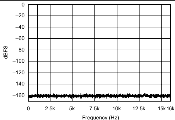
Figure 25. FFT With 1 kHz Input Tone at 0 dBFS (192 kHz:32 kHz)
