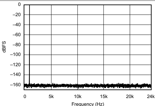
Figure 29. FFT With 1 kHz Input Tone at 0 dBFS (192 kHz:48 kHz)
