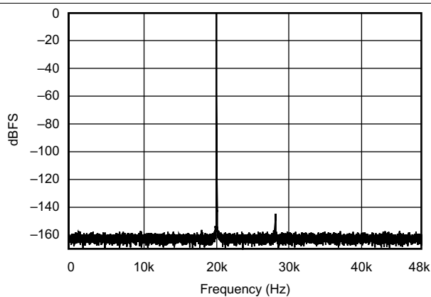
Figure 35. FFT With 20 kHz Input Tone at 0 dBFS (48 kHz:96 kHz)
