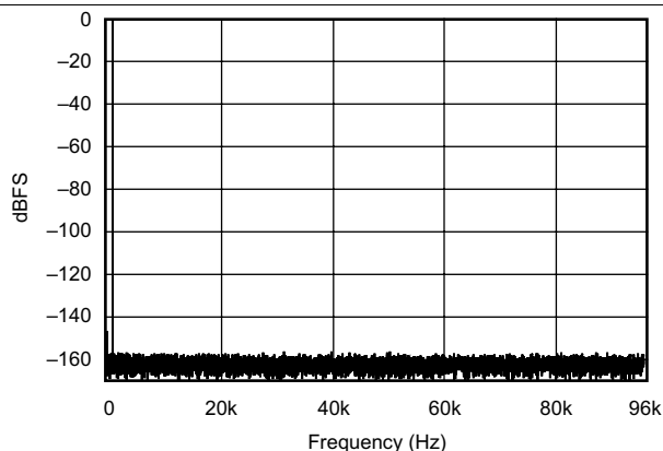
Figure 1. FFT With 1 kHz Input Tone at 0 dBFS (12 kHz:192 kHz)
