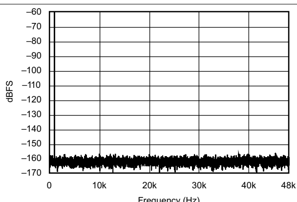
Figure 72. FFT With 1 kHz Input Tone at -60 dBFS (44.1 kHz:96 kHz)
