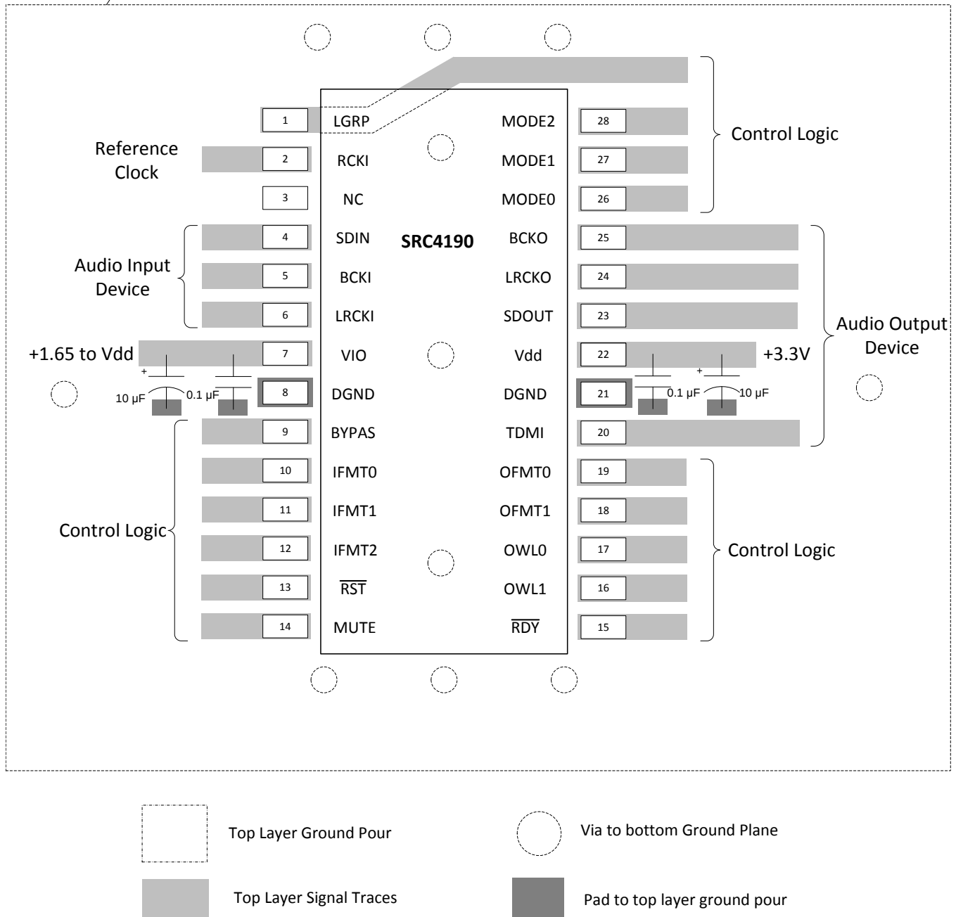
Figure 73. Diagram of an Example Layout
