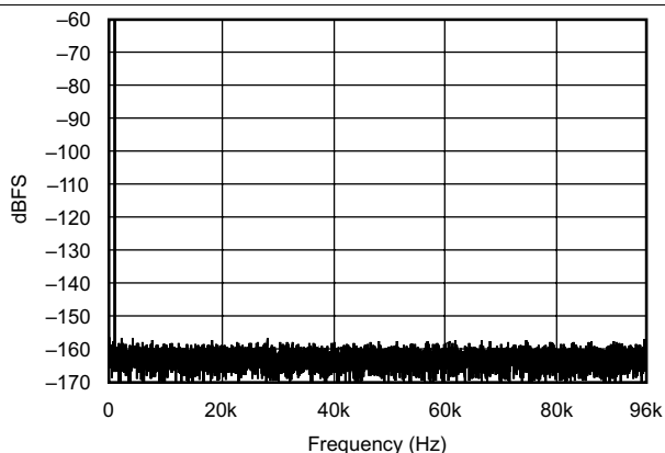
Figure 2. FFT With 1 kHz Input Tone at -60 dBFS (12 kHz:192 kHz)
