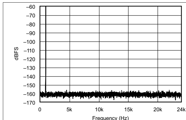
Figure 71. FFT With 1 kHz Input Tone at -60 dBFS (44.1 kHz:48 kHz)
