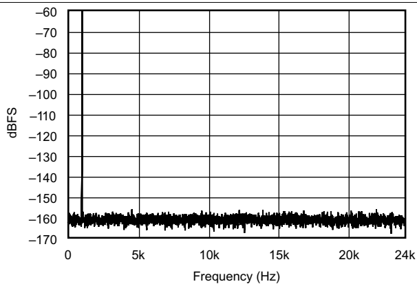
Figure 6. FFT With 1 kHz Input Tone at -60 dBFS (44.1 kHz:48 kHz)
