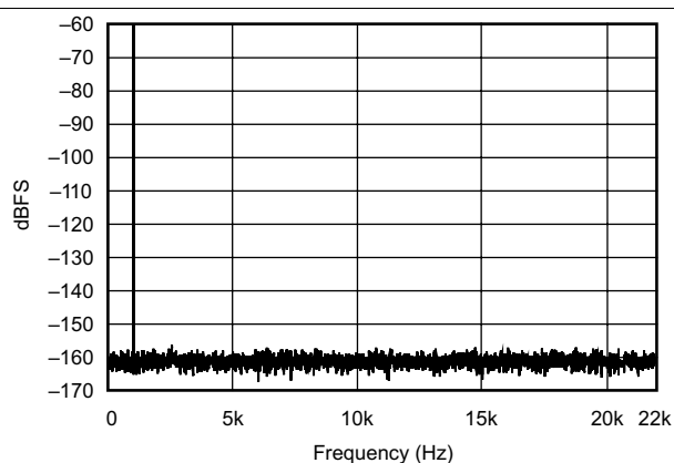
Figure 18. FFT With 1 kHz Input Tone at -60 dBFS (96 kHz:44.1 kHz)
