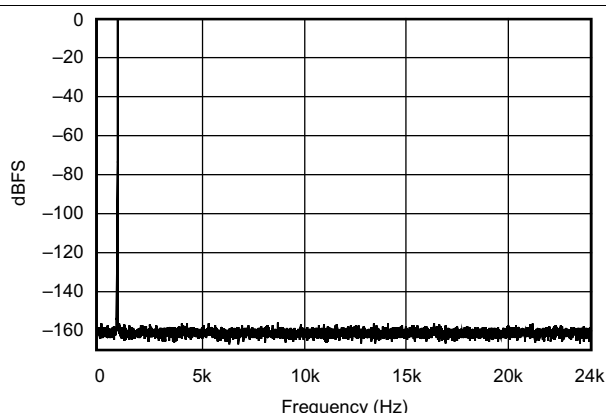
Figure 3. FFT With 1 kHz Input Tone at 0 dBFS (32 kHz:48 kHz)
