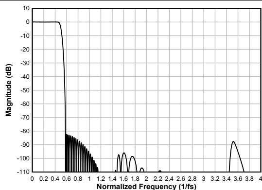
Figure 6-21. Linear-phase Decimation Filter Magnitude Response
