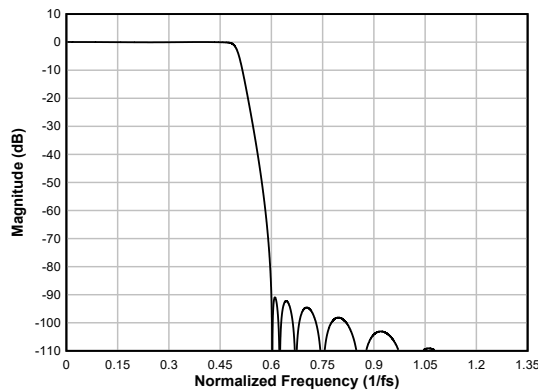
Figure 6-35. Low-latency Decimation Filter Magnitude Response
