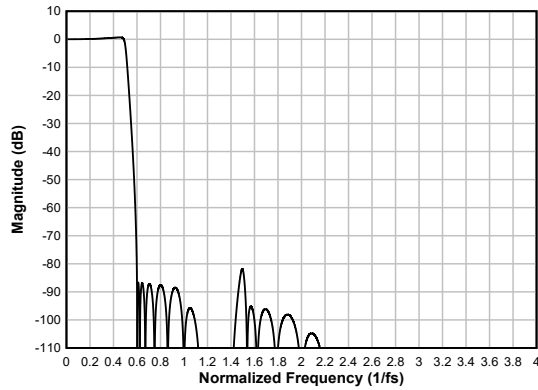
Figure 6-27. Low-latency Decimation Filter Magnitude Response
