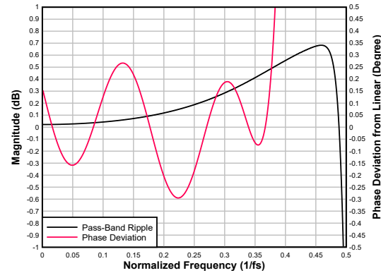
Figure 6-28. Low-latency Decimation Filter Pass-Band Ripple and Phase Deviation
