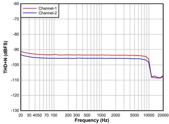
Figure 5-8. ADC THD+N vs Frequency
