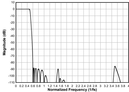
Figure 6-33. Low-latency Decimation Filter Magnitude Response
