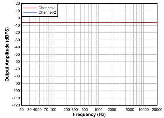
Figure 5-9. ADC Frequency Response
