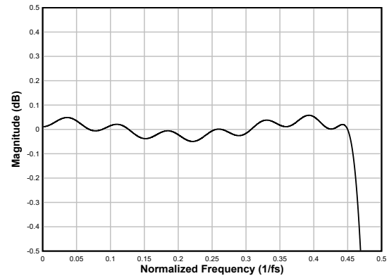
Figure 6-24. Linear-phase Decimation Filter Pass-Band Ripple
