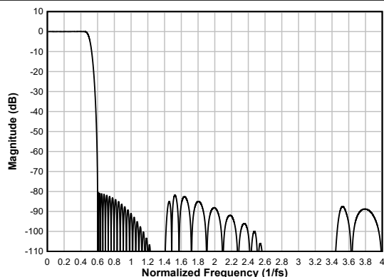
Figure 6-19. Linear-phase Decimation Filter Magnitude Response
