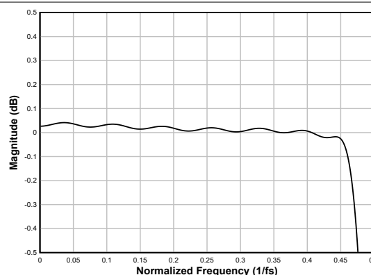
Figure 6-14. Linear-phase Decimation Filter Pass-Band Ripple
