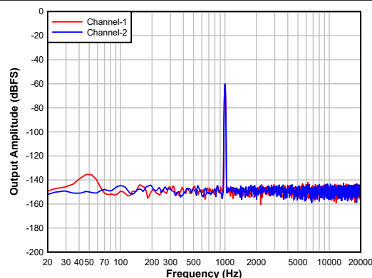
Figure 7-3. ADC FFT with -60dBFS Input
