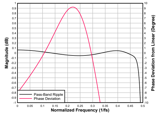
Figure 6-57. Low-latency Decimation Filter Pass-Band Ripple and Phase Deviation
