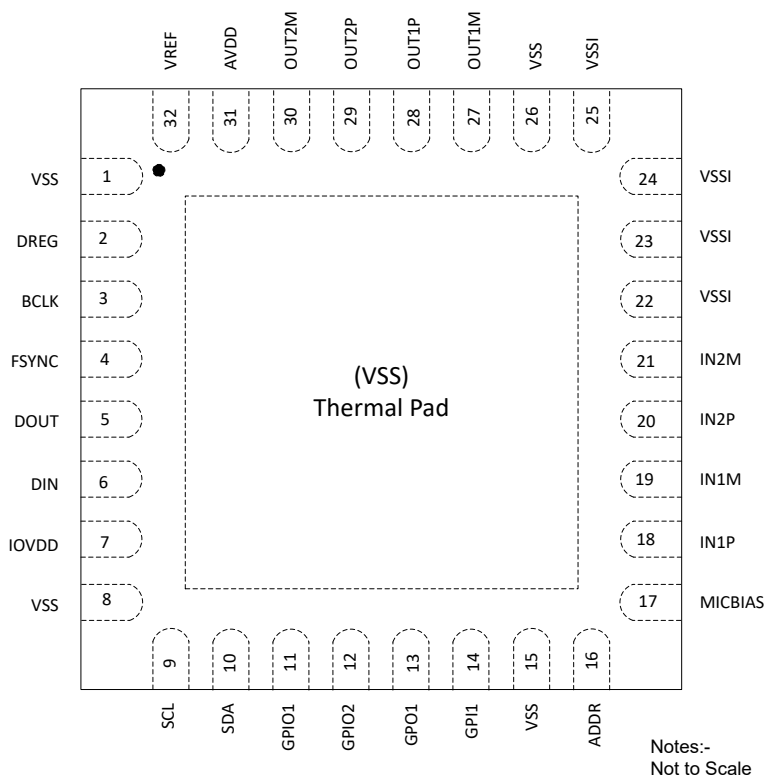
Figure 4-1. TAC5112-Q1 RTV Package, 32-Pin WQFN With Exposed Thermal Pad, Top View
