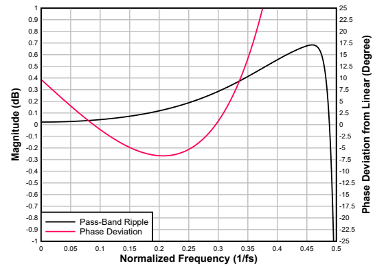
Figure 6-61. Ultra Low-latency Decimation Filter Pass-Band Ripple and Phase Deviation
