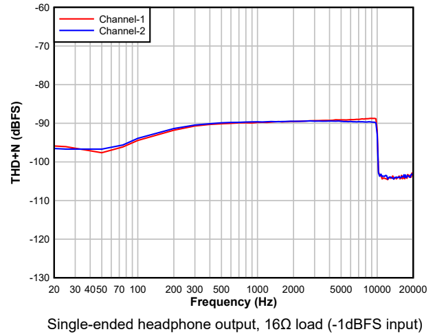
Figure 5-28. DAC THD+N Level vs Frequency
