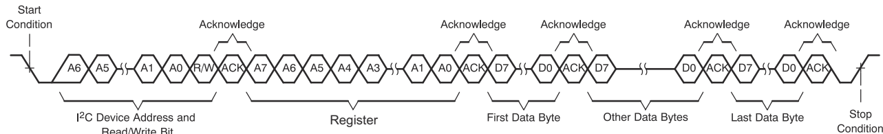
Figure 6-111. I 2 C Multiple-Byte Write Transfer
