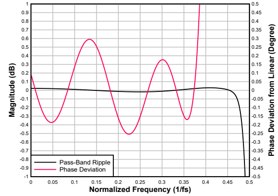
Figure 6-55. Low-latency Decimation Filter Pass-Band Ripple and Phase Deviation
