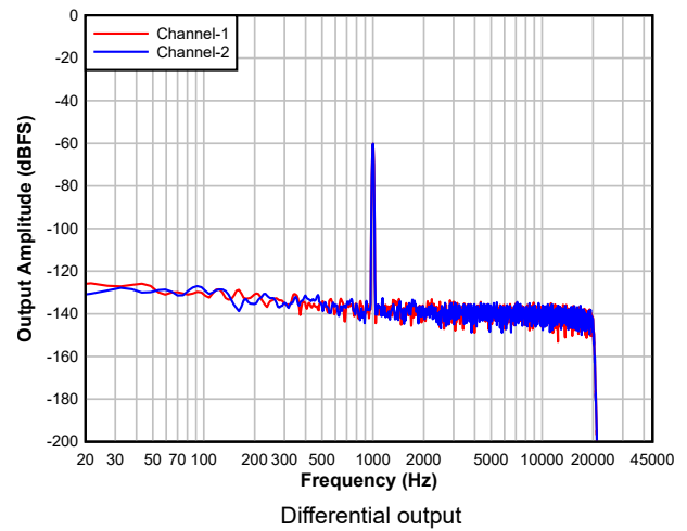
Figure 5-30. DAC FFT with -60dBFS Input
