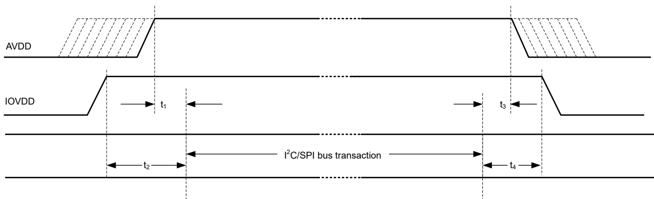
Figure 8-6. Power-Supply Sequencing Requirement Timing Diagram
