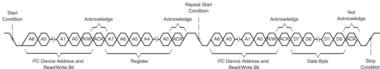
Figure 6-112. I 2 C Single-Byte Read Transfer
