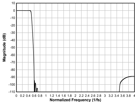
Figure 6-93. Low-latency Interpolation Filter Magnitude Response
