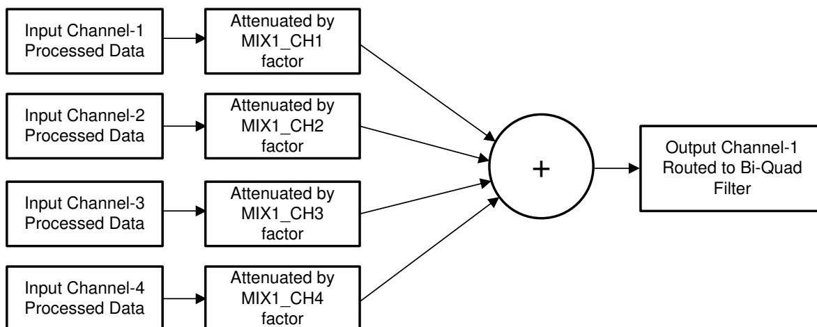
Figure 6-29. Programmable Digital Mixer Block Diagram
