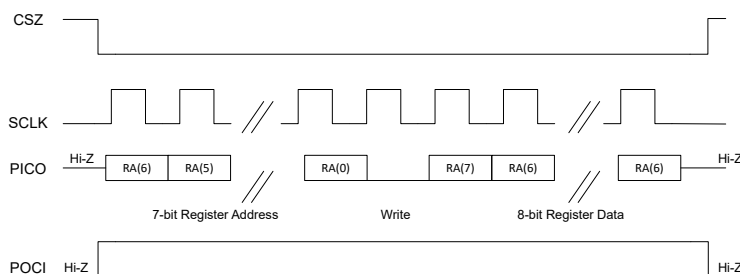
Figure 6-114. SPI Single-Byte Write Transfer
