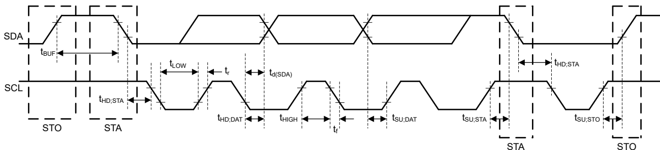
Figure 5-1. I²C Interface Timing Diagram
