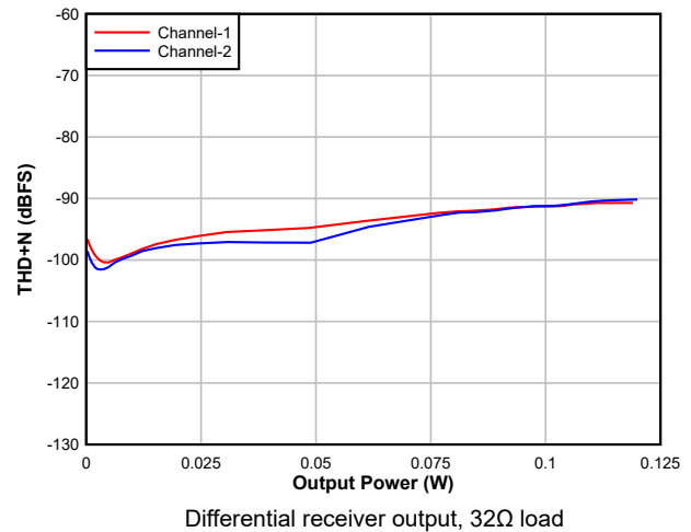
Figure 5-22. DAC THD+N Level vs output power
