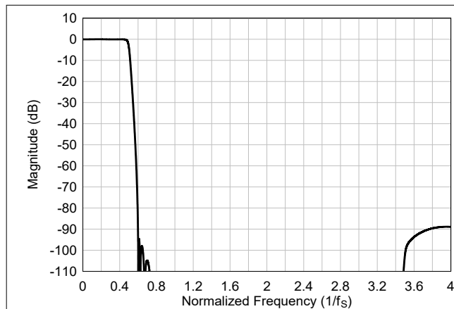
Figure 6-103. Ultra-Low-Latency interpolation Filter Magnitude Response
