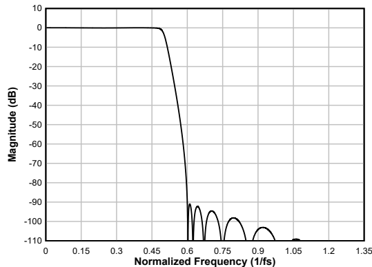
Figure 6-56. Low-latency Decimation Filter Magnitude Response
