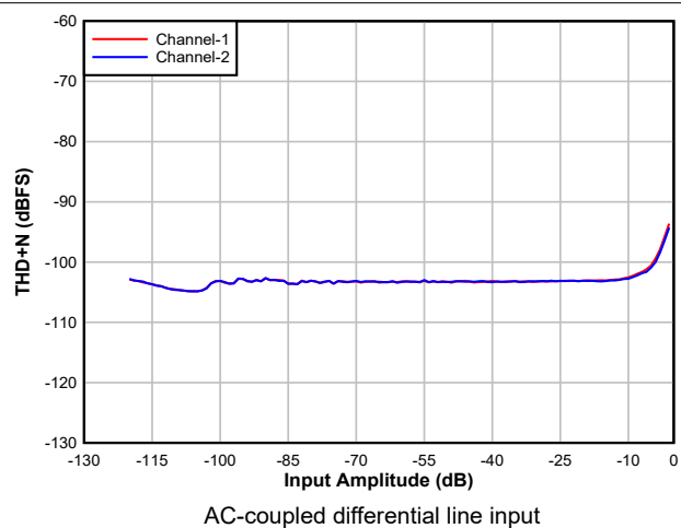
Figure 8-3. ADC THD+N Level vs Input
