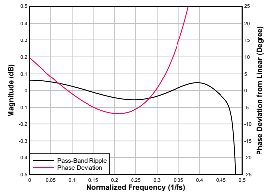
Figure 6-67. Ultra Low-latency Decimation Filter Pass-Band Ripple and Phase Deviation
