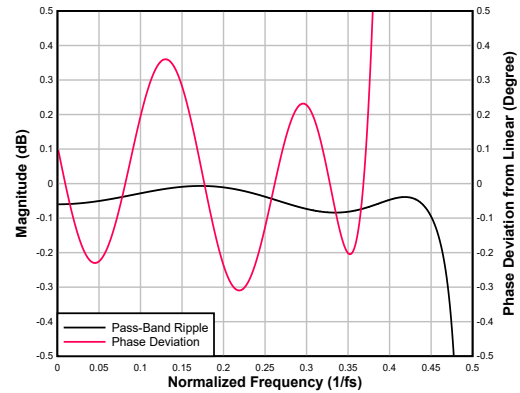
Figure 6-94. Low-latency Interpolation Filter Pass-Band Ripple and Phase Deviation
