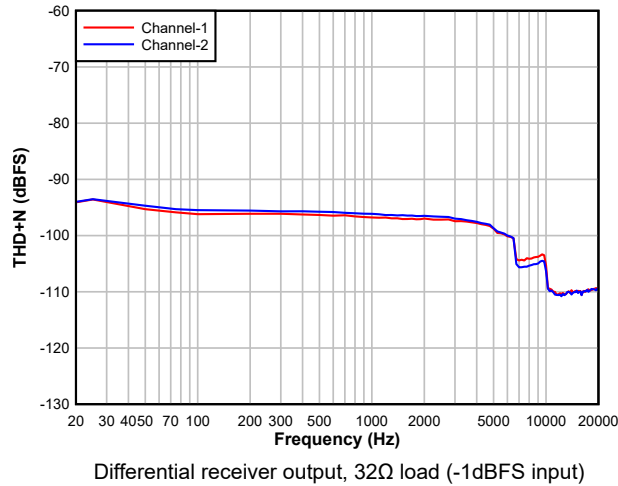
Figure 5-27. DAC THD+N Level vs Frequency
