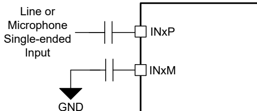
Figure 6-17. Single-ended AC-Coupled Input Connection (ADC_CHx_INSRC set to 2'b01 and ADC_CHx_CM_TOL set to 2'b00 or 2'b01 or 2'10)
