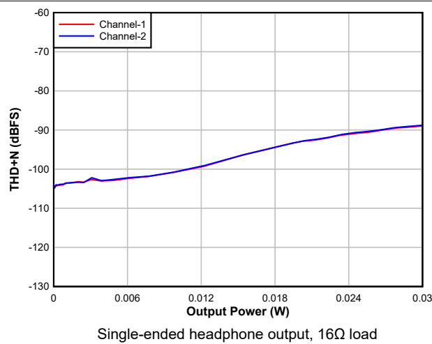
Figure 5-23. DAC THD+N Level vs output power
