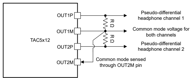
Figure 6-23. Psuedo-differential Output Connection with External Common-Mode Sense (OUT1x_CFG[2:0] = 3'b101)
