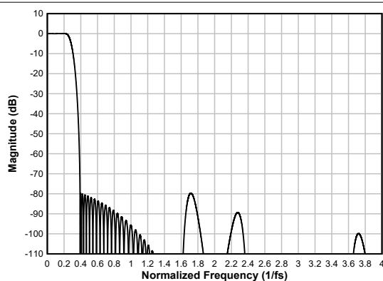
Figure 6-44. Linear-phase Decimation Filter Magnitude Response
