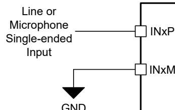
Figure 6-18. Single-ended DC-Coupled Input Connection (ADC_CHx_INSRC set to 2'b01 and ADC_CHx_CM_TOL set to 2'b01 or 2'10)
