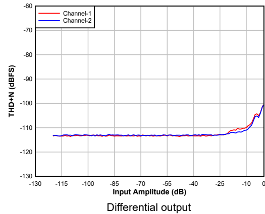
Figure 8-5. DAC THD+N Level vs Input
