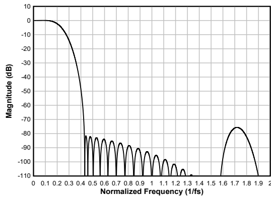
Figure 6-46. Linear-phase Decimation Filter Magnitude Response
