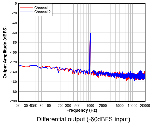
Figure 8-4. DAC FFT with -60dBFS Input
