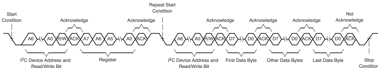
Figure 6-113. I 2 C Multiple-Byte Read Transfer
