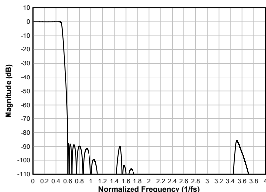
Figure 6-64. Ultra Low-latency Decimation Filter Magnitude Response
