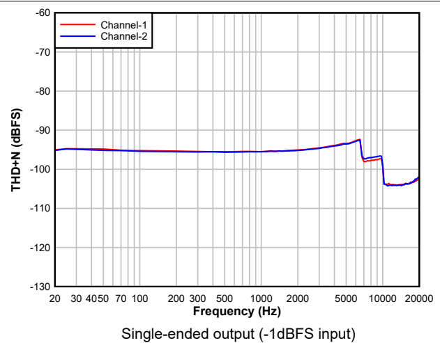
Figure 5-26. DAC THD+N Level vs Frequency
