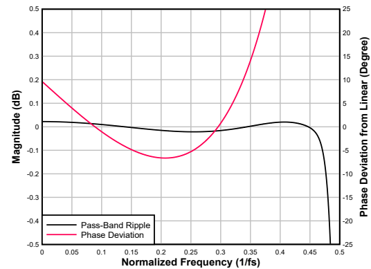
Figure 6-63. Ultra Low-latency Decimation Filter Pass-Band Ripple and Phase Deviation
