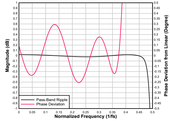
Figure 6-53. Low-latency Decimation Filter Pass-Band Ripple and Phase Deviation
