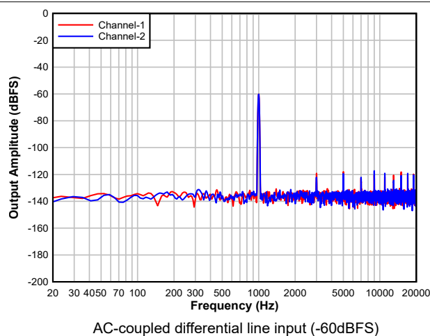
Figure 8-2. ADC FFT with -60dBFS Input
