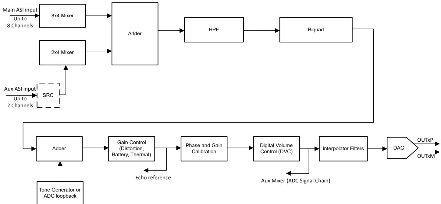
Figure 6-69. DAC Signal-Chain Processing Flowchart
