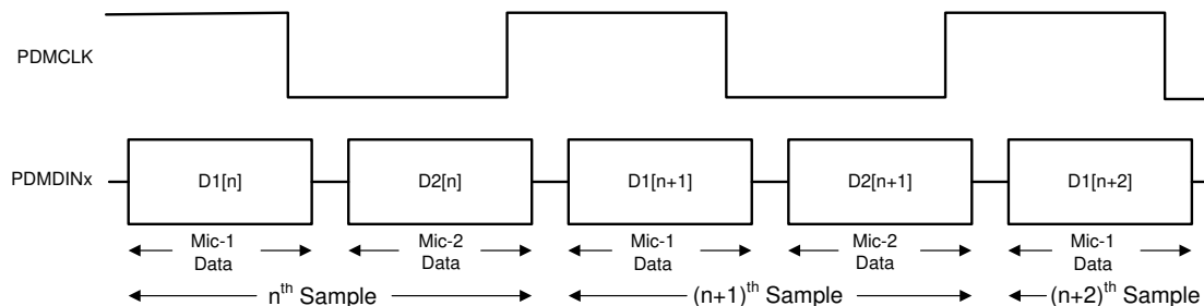
Figure 6-26. Digital PDM Microphone Protocol Timing Diagram
