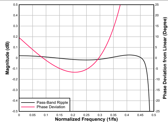
Figure 6-65. Ultra Low-latency Decimation Filter Pass-Band Ripple and Phase Deviation
