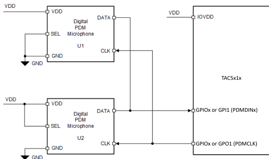
Figure 6-25. Digital PDM Microphones Connection Diagram for the TAC5112-Q1
