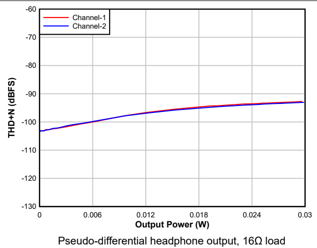
Figure 5-24. DAC THD+N Level vs output power
