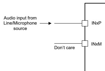
Figure 6-20. Single-ended mux on INxP DC-Coupled Input Connection (ADC_CHx_INSRC set to 2'b10 and ADC_CHx_CM_TOL set to 2'b01 or 2'10)
