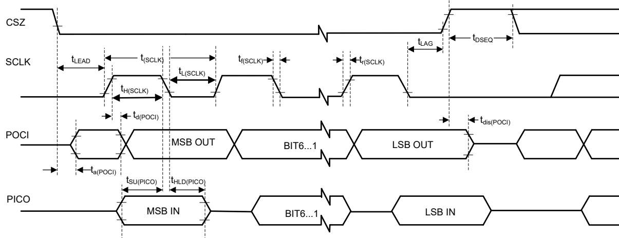
Figure 5-2. SPI Timing Diagram
