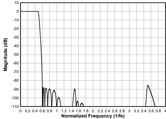
Figure 6-54. Low-latency Decimation Filter Magnitude Response
