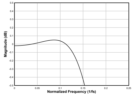
Figure 6-47. Linear-phase Decimation Filter Pass-Band Ripple
