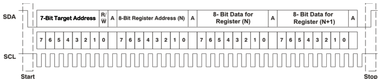
Figure 6-109. Typical I 2 C Sequence
