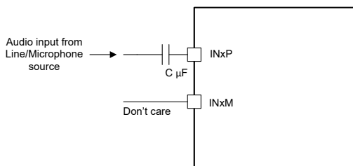
Figure 6-19. Single-ended mux on INxP AC-Coupled Input Connection (ADC_CHx_INSRC set to 2'b10 and ADC_CHx_CM_TOL set to 2'b00 or 2'b01 or 2'10)
