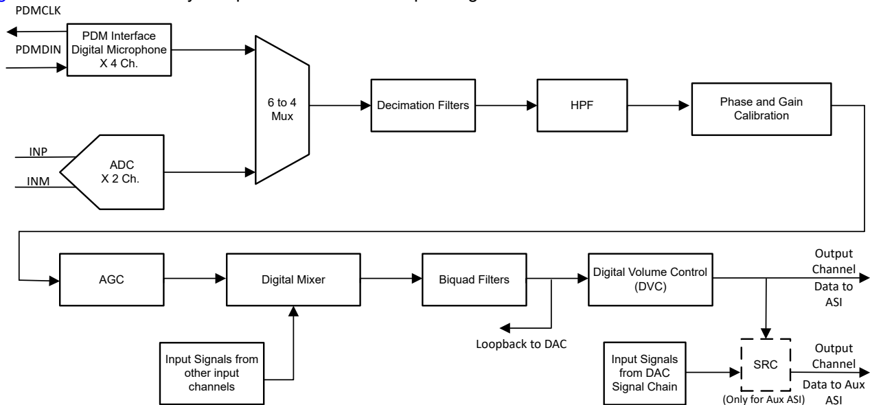
Figure 6-27. ADC Signal-Chain Processing Flowchart
