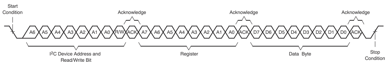
Figure 6-110. I 2 C Single-Byte Write Transfer
