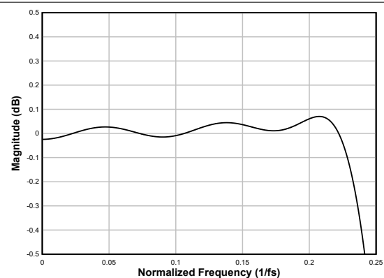
Figure 6-45. Linear-phase Decimation Filter Pass-Band Ripple
