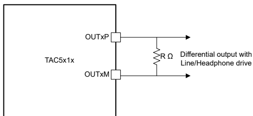
Figure 6-21. Differential Output Connection (OUT1x_CFG[2:0] = 3'b000)
