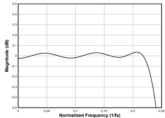
Figure 6-43. Linear-phase Decimation Filter Pass-Band Ripple
