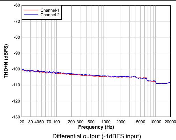
Figure 5-25. DAC THD+N Level vs Frequency
