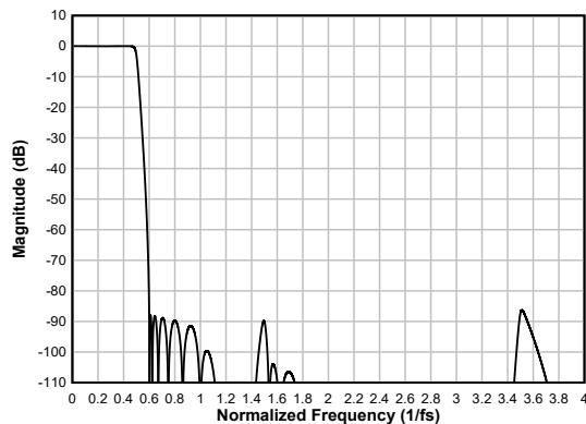
Figure 6-62. Ultra Low-latency Decimation Filter Magnitude Response
