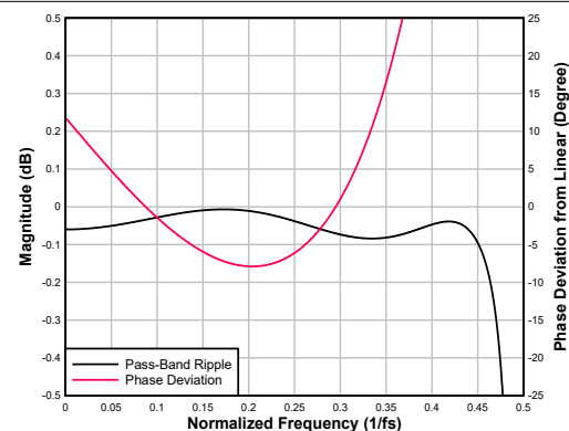
Figure 6-104. Ultra-Low-Latency interpolation Filter Pass-Band Ripple and Phase Deviation
