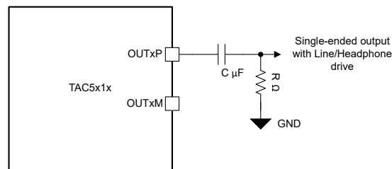
Figure 6-22. Mono Single-ended Output Connection on OUT1P (OUT1x_CFG[2:0] = 3'b010)
