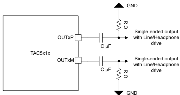
Figure 6-24. Stereo Single-ended Output Connection (OUT1x_CFG[2:0] = 3'b001)
