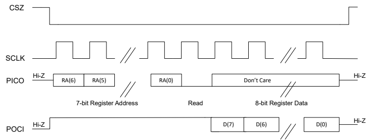
Figure 6-115. SPI Single-Byte Read Transfer
