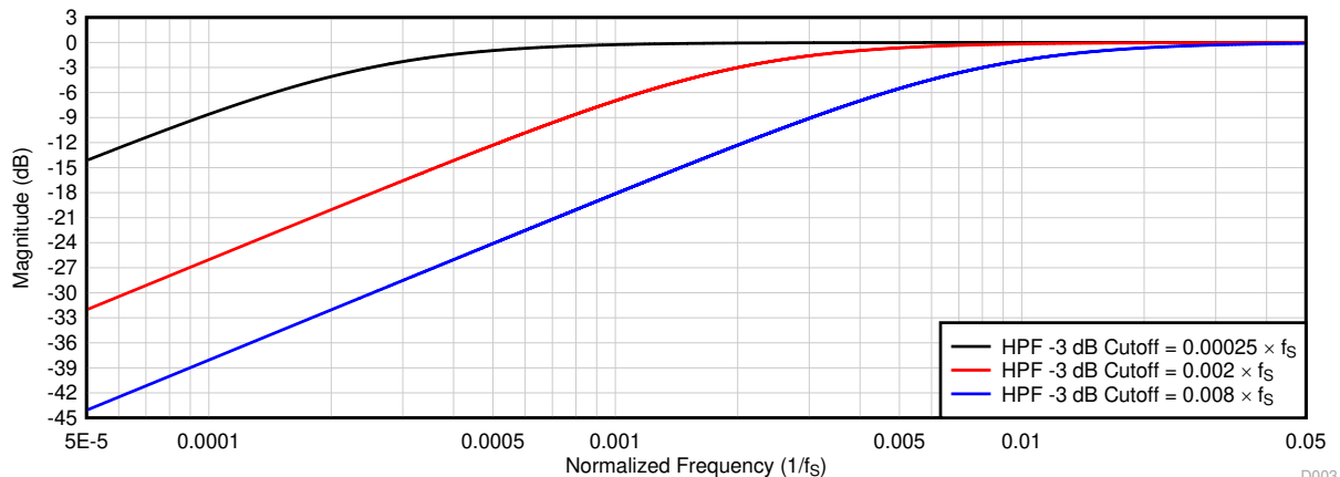
Figure 6-28. HPF Filter Frequency Response Plot
