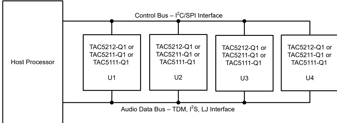
Figure 6-14. Multiple TAC5112-Q1 Devices With Shared Control and Audio Data Buses
