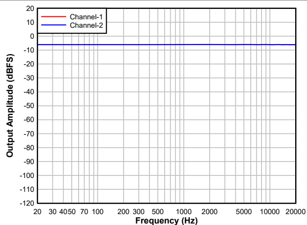
Figure 5-34. DAC Frequency Response
