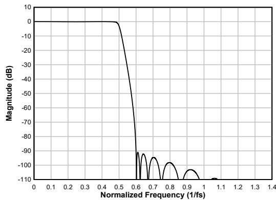
Figure 6-66. Ultra Low-latency Decimation Filter Magnitude Response
