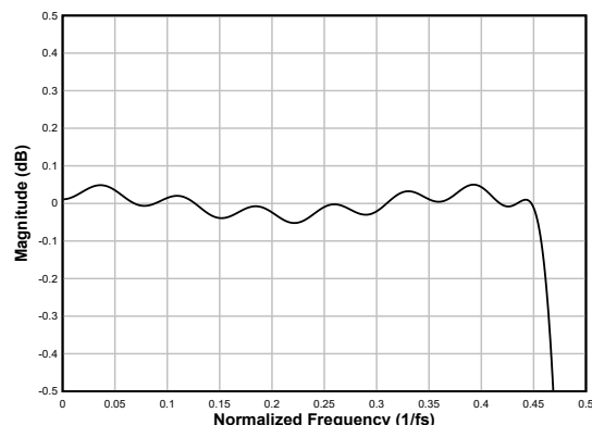
Figure 6-71. Linear-phase Decimation Filter Pass-Band Ripple
