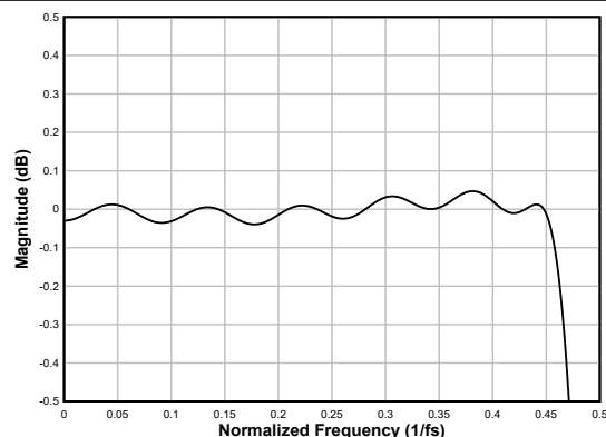
Figure 6-69. Linear-phase Decimation Filter Pass-Band Ripple
