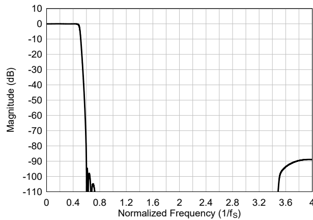
Figure 6-54. Ultra-Low-Latency interpolation Filter Magnitude Response
