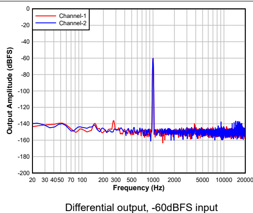
Figure 7-3. DAC FFT
