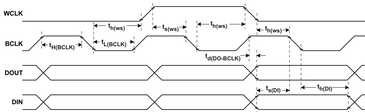
Figure 43. DSP Timing in Slave Mode
