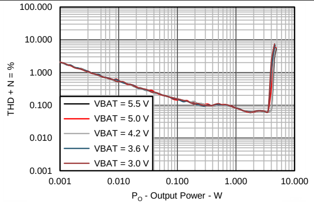
Figure 16. I-Sense THD+N vs Output Power (6Ω)
