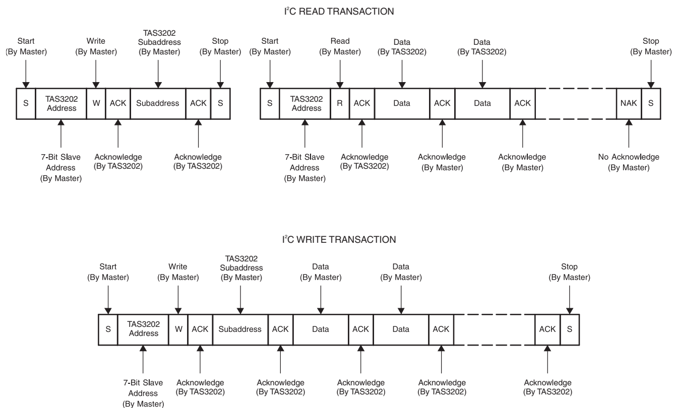
Figure 6-3. I 2 C Subaddress Access Protocol
