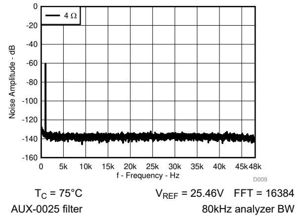
Figure 6-12. Noise vs Frequency
