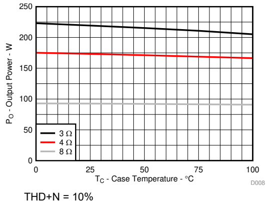
Figure 6-11. Output Power vs Temperature
