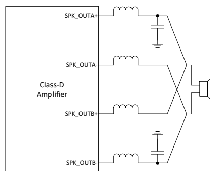
Figure 7-20. Post-Filter PBTL
