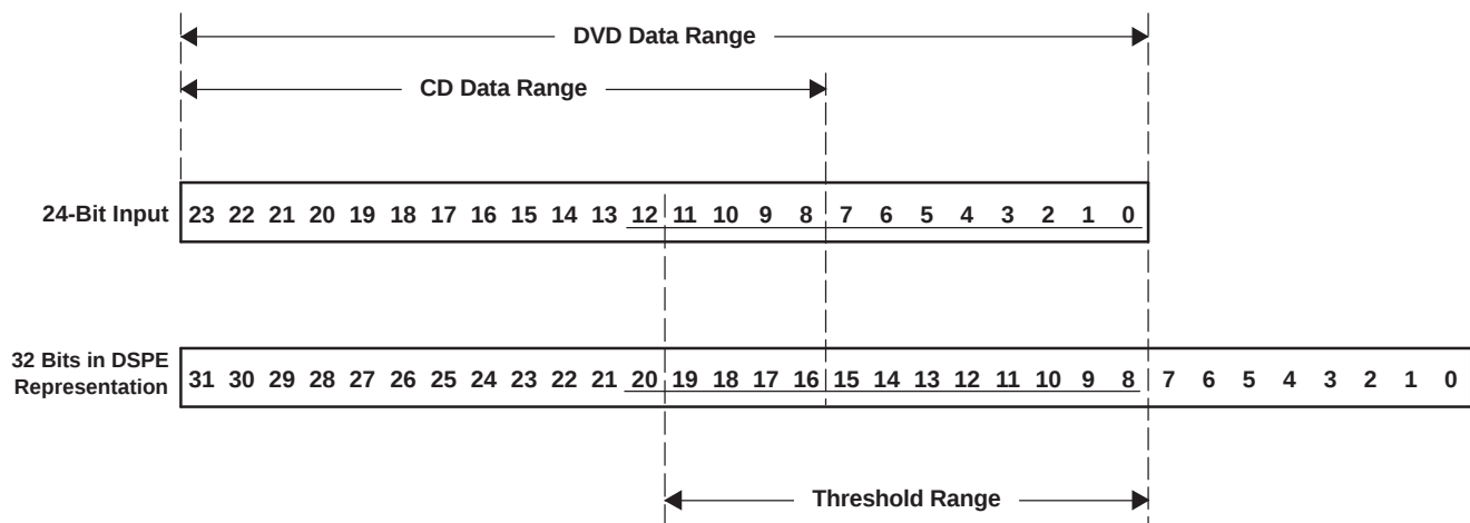
Figure 1-14. Automute Threshold
