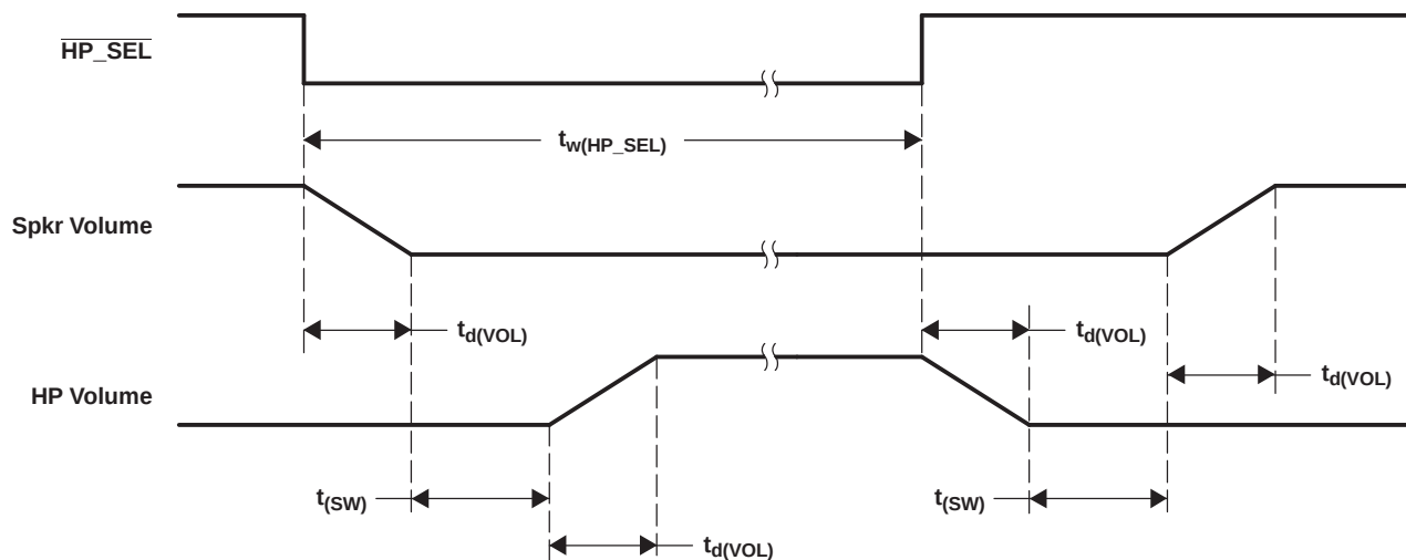
Figure 4-9. \overline{\text{HP\_SEL}} Timing
