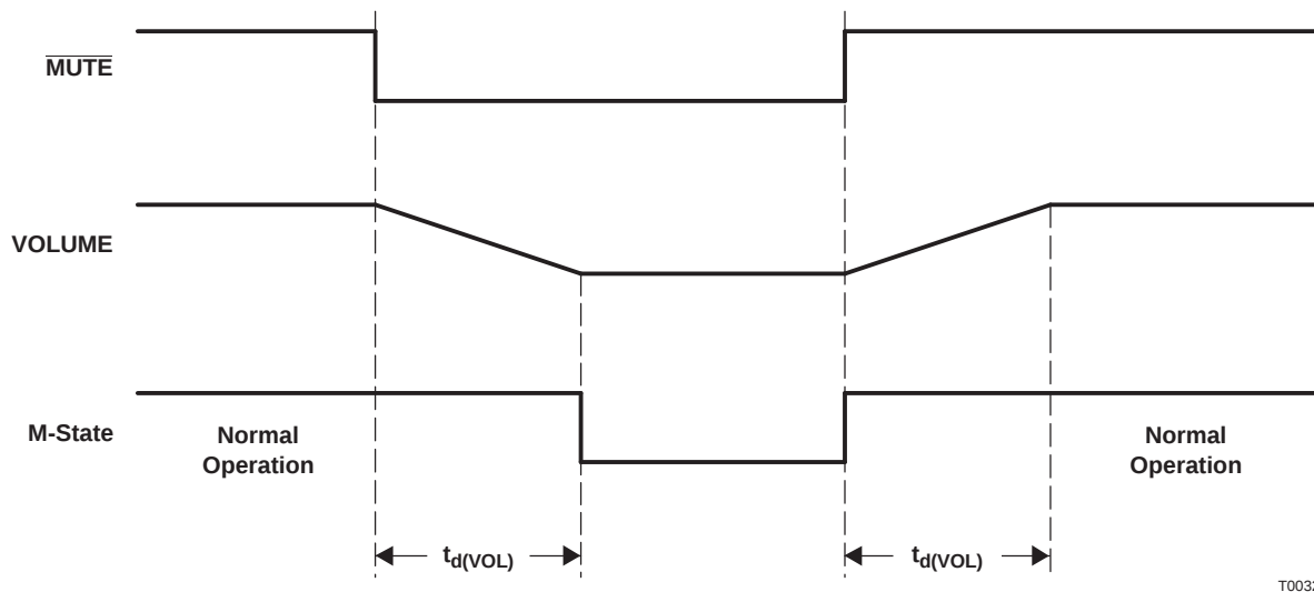
Figure 4-7. Mute Timing
