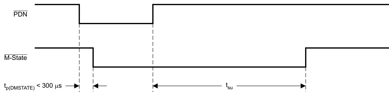
Figure 4-5. Power-Down Timing
