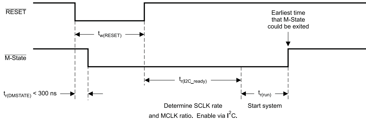
Figure 4-4. Reset Timing
