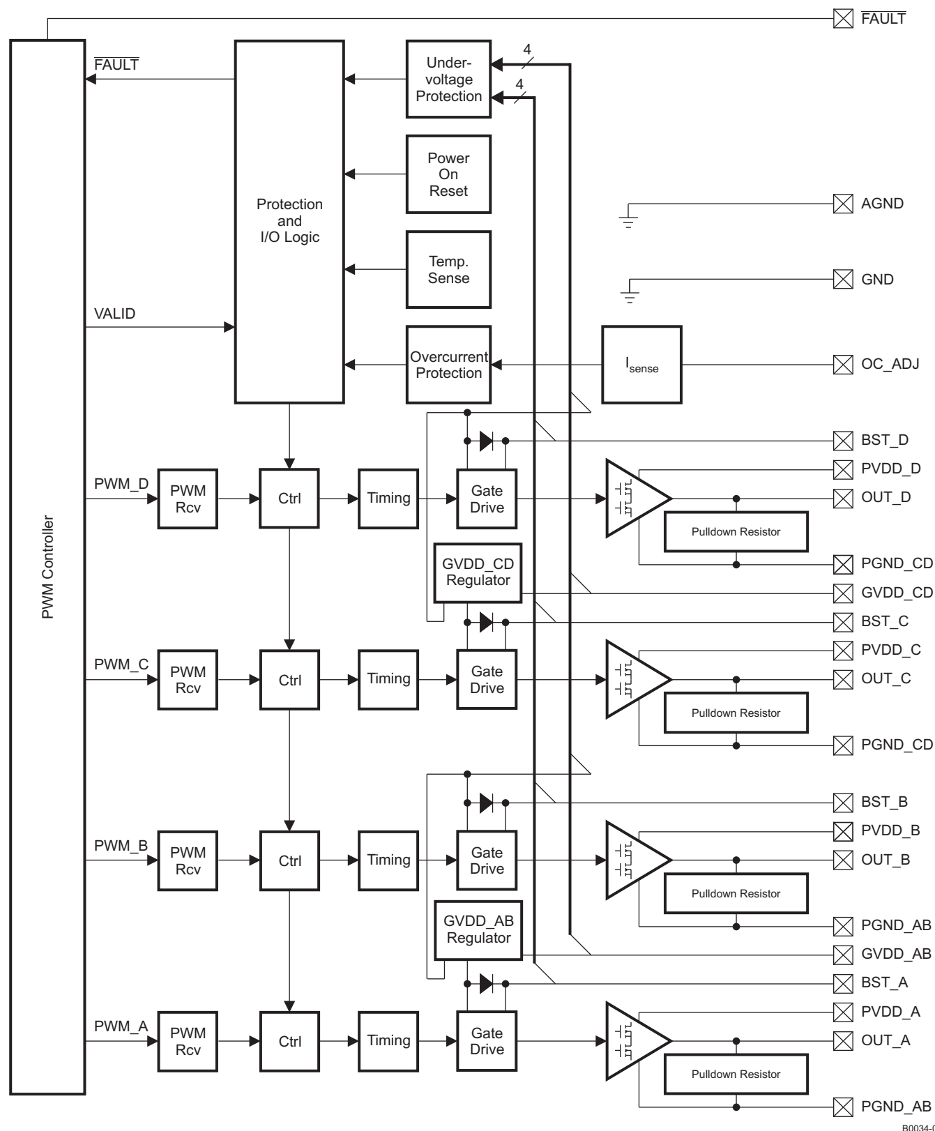
Figure 1. Power Stage Functional Block Diagram
