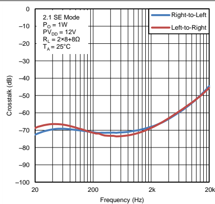
Figure 14. Crosstalk vs Frequency (2.1 SE Mode)
