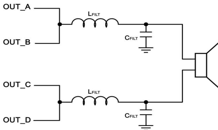
Figure 58. Post-Filter PBTL
