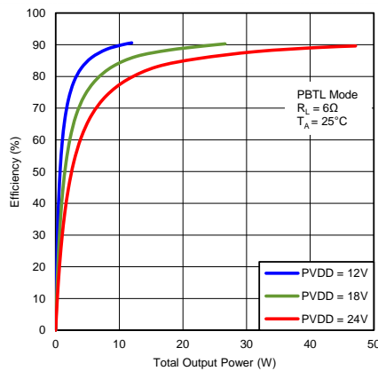
Figure 40. Efficiency vs Output Power (PBTL Mode)
