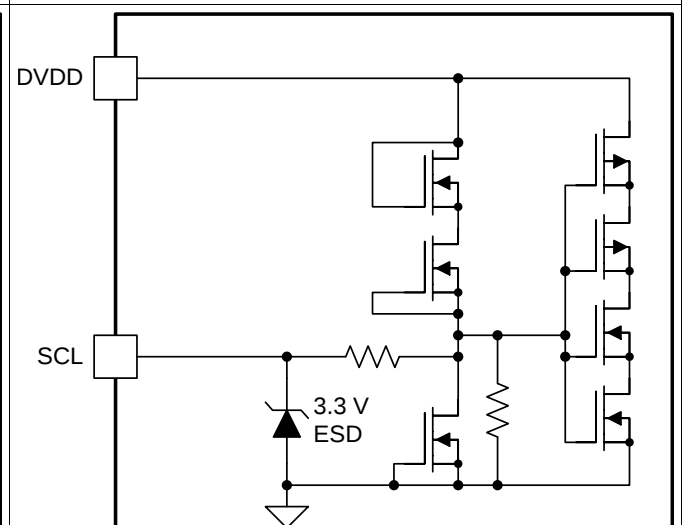
Figure 12. SCL Pin
