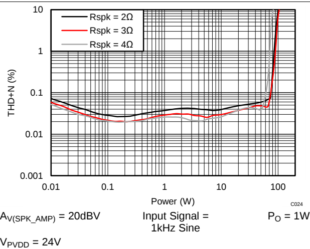
Figure 52. THD+N vs Power – PBTL
