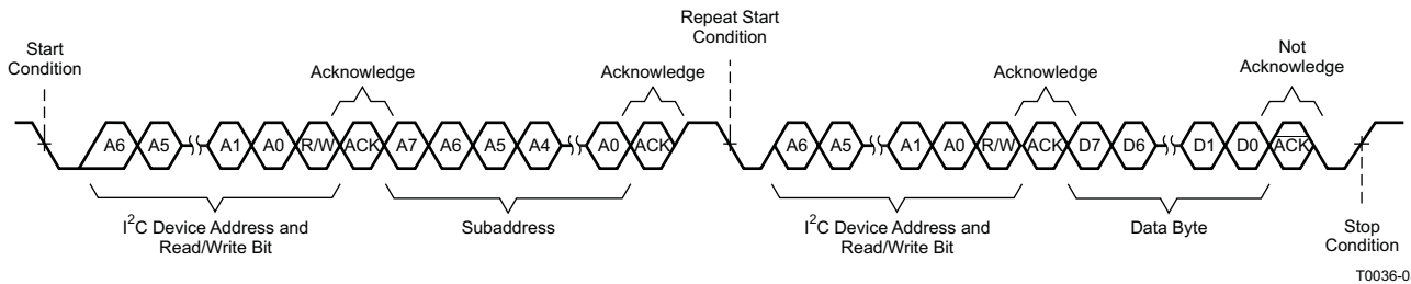
Figure 46. Read Transfer
