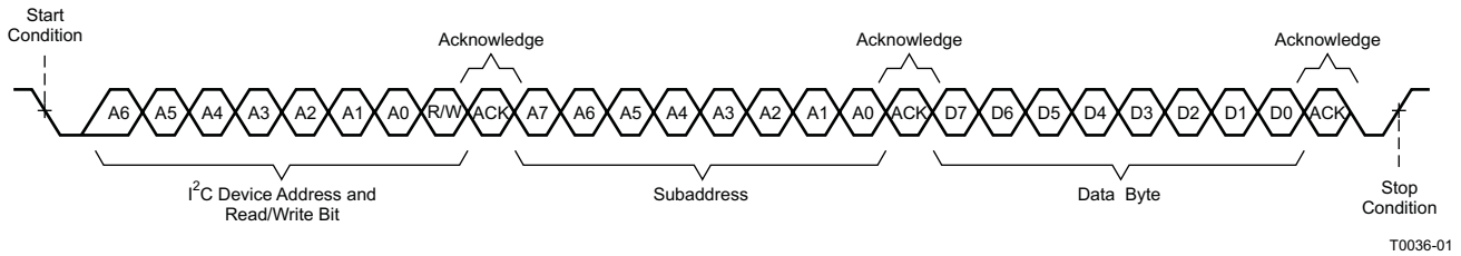
Figure 45. Write Transfer
