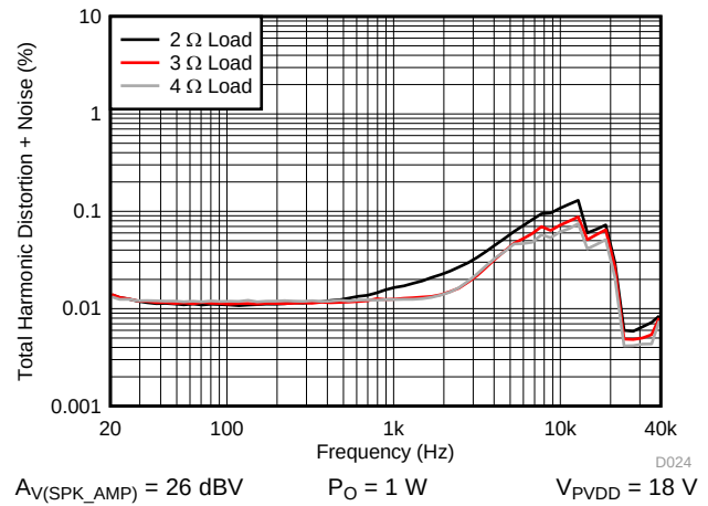
Figure 46. THD+N vs Frequency – PBTB
