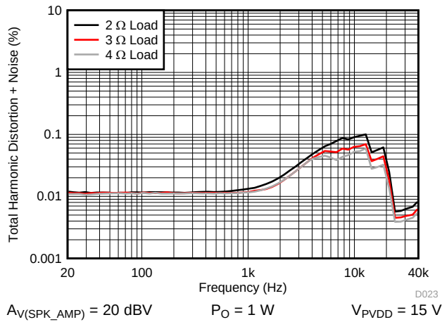
Figure 45. THD+N vs Frequency – PBTB
