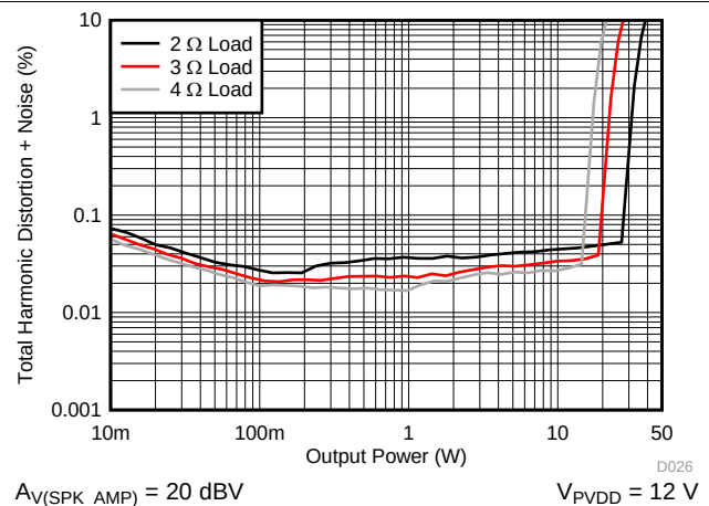
Figure 48. THD+N vs Power – PBTB
