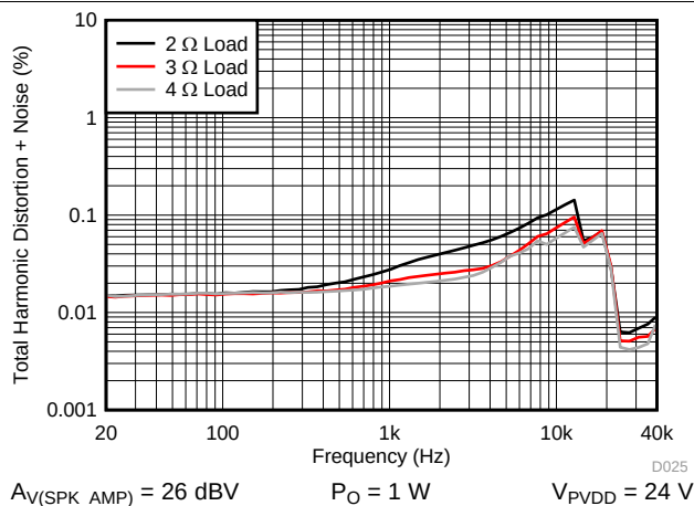
Figure 47. THD+N vs Frequency – PBTB
