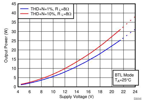
Figure 6-48. Output Power vs Supply Voltage
