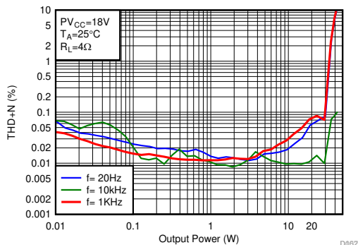
Figure 6-73. THD+N vs Output Power-PBTL
