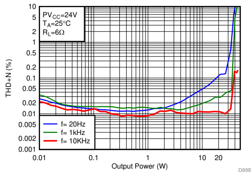
Figure 6-19. THD+N vs Output Power-BTL
