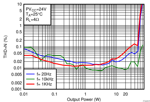
Figure 6-74. THD+N vs Output Power-PBTL
