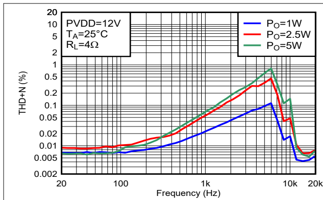
Figure 5-20. THD+N vs Frequency-BTL
