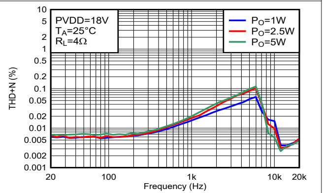
Figure 5-42. THD+N vs Frequency-PBTL
