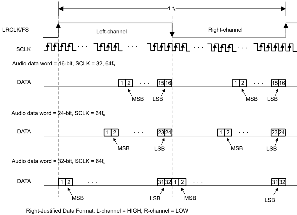
Right Justified Data Format; L-channel = HIGH, R-channel = LOW
