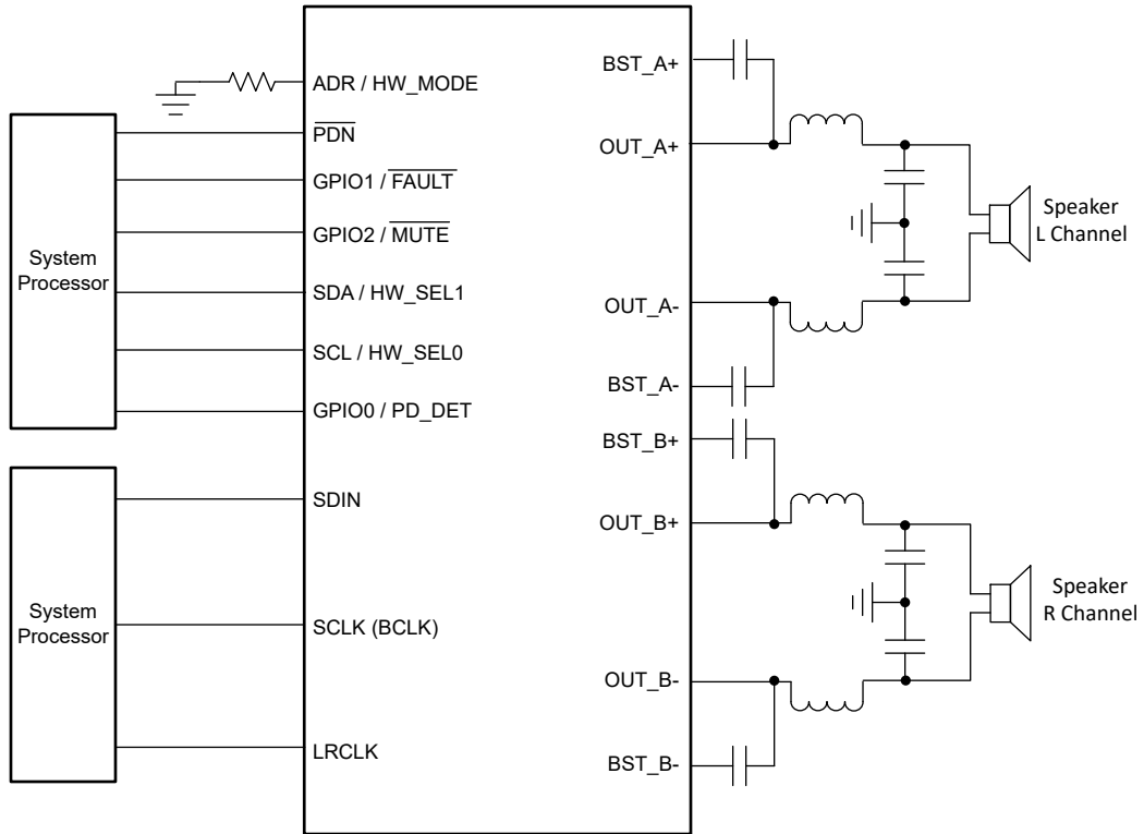
Simplified Schematic
