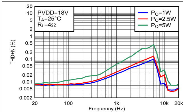
Figure 5-22. THD+N vs Frequency-BTL
