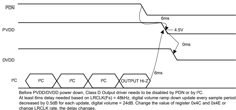
Figure 6-17. Power-Down Sequence
