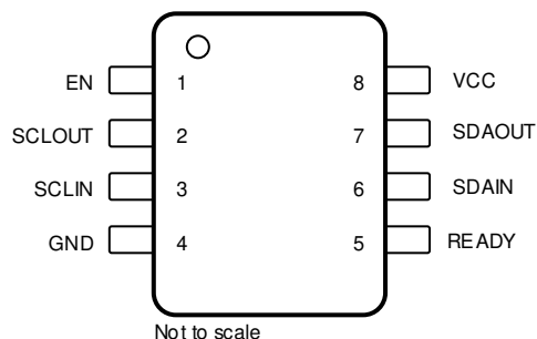
Figure 4-1. 8-Pin VSSOP, DKG Package (Top View)
