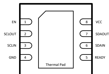
Figure 4-2. 8-Pin WSON, DRG Package (Top View)
