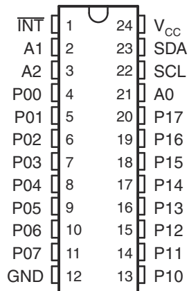
Figure 4-1. DB, PW (TSSOP) Package 24-Pin (Top View)
