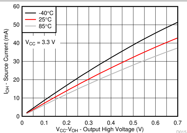
Figure 5-14. I/O Source Current vs Output High Voltage for Different Temperature ( T_A ) for V_{CC} = 3.3\text{V}
