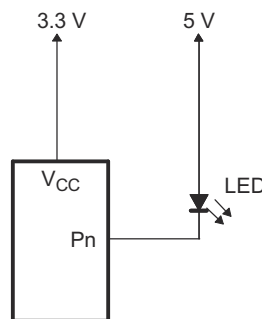
Figure 7-3. Device Supplied by Lower Voltage
