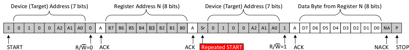
Figure 6-8. Read from Register
