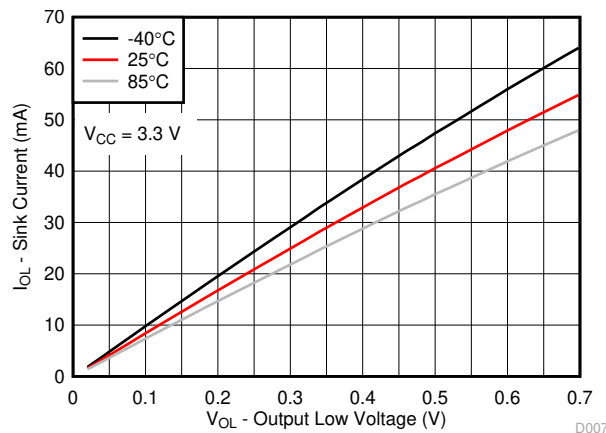
Figure 5-7. I/O Sink Current vs Output Low Voltage for Different Temperature ( T_A ) for V_{CC} = 3.3\text{V}
