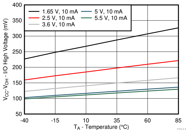
Figure 5-17. V_{CC} - V_{OH} Voltage vs Temperature for Different V_{CC}
