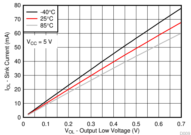
Figure 5-8. I/O Sink Current vs Output Low Voltage for Different Temperature ( T_A ) for V_{CC} = 5\text{V}
