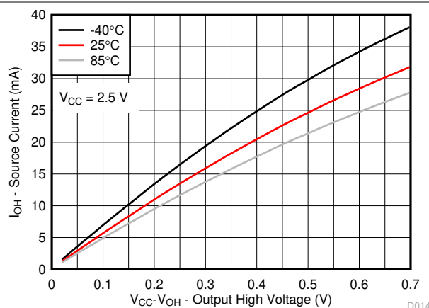
Figure 5-13. I/O Source Current vs Output High Voltage for Different Temperature ( T_A ) for V_{CC} = 2.5\text{V}
