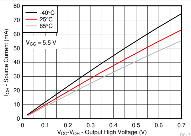
Figure 5-16. I/O Source Current vs Output High Voltage for Different Temperature ( T_A ) for V_{CC} = 5.5\text{V}
