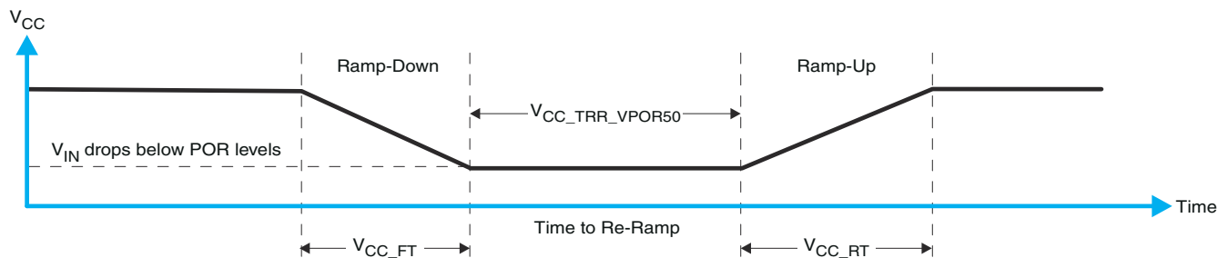
Figure 7-7. V_{CC} Is Lowered Below The Por Threshold, Then Ramped Back Up To V_{CC}
