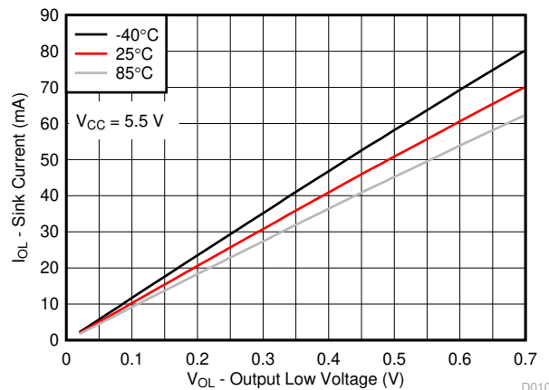
Figure 5-9. I/O Sink Current vs Output Low Voltage for Different Temperature ( T_A ) for V_{CC} = 5.5\text{V}
