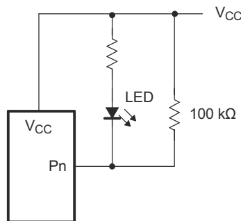
Figure 7-2. High-Value Resistor in Parallel With LED
