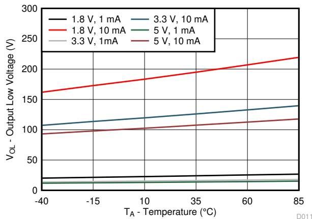
Figure 5-10. I/O Low Voltage vs Temperature for Different V_{CC} and I_{OL}
