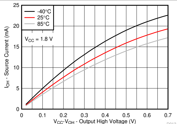
Figure 5-12. I/O Source Current vs Output High Voltage for Different Temperature ( T_A ) for V_{CC} = 1.8\text{V}
