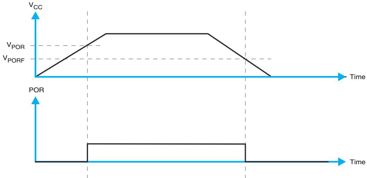
Figure 7-9. V_{POR}
