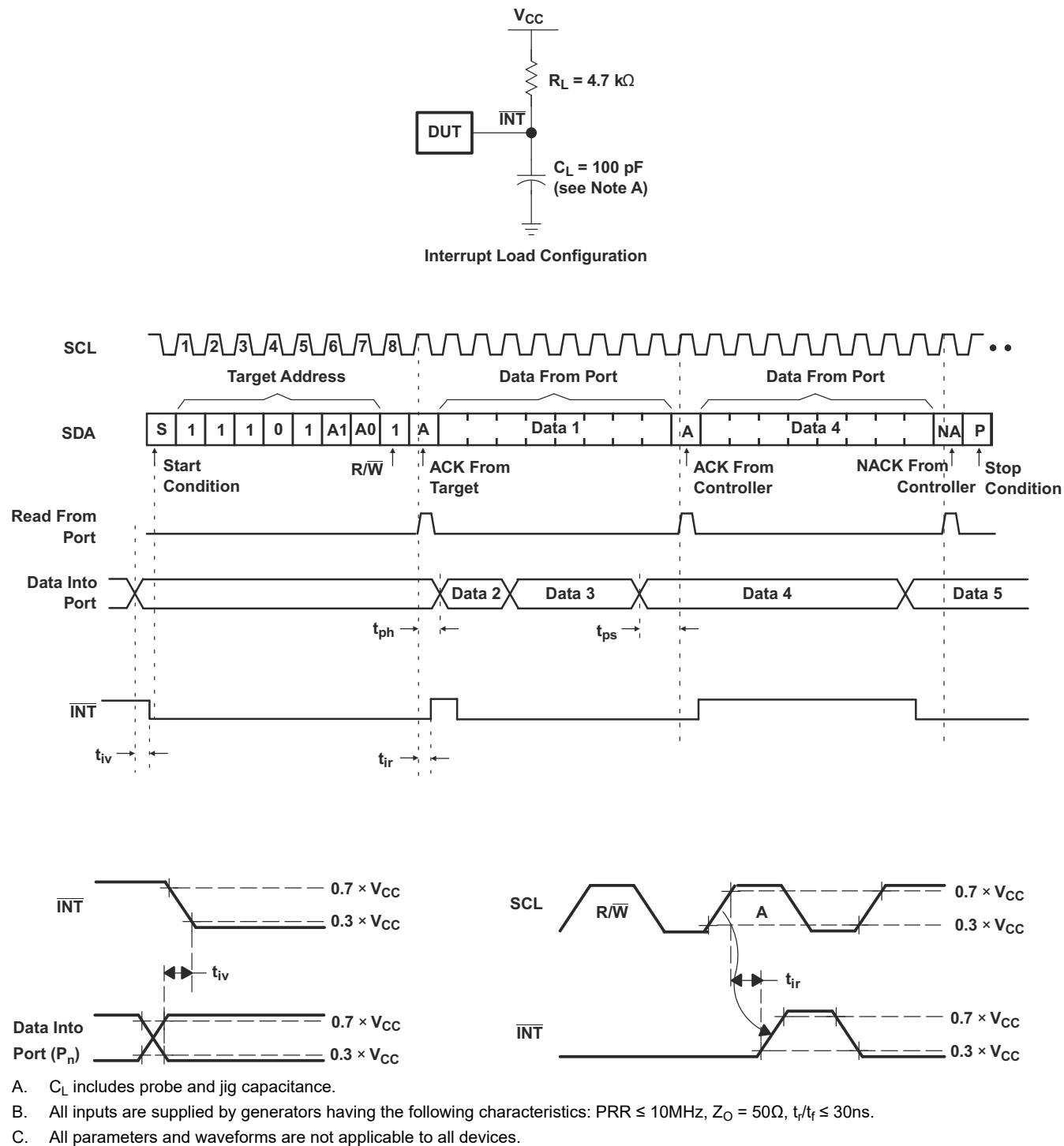
Figure 6-2. Interrupt Load Circuit and Voltage Waveforms
