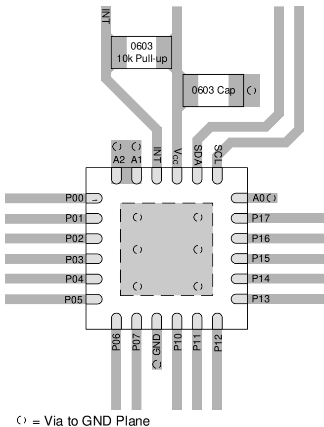
Figure 7-10. TCA9535 Layout Example
