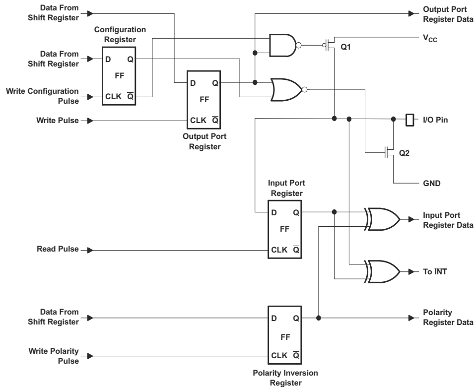
Figure 6-2. Simplified Schematic of P-Port I/Os
