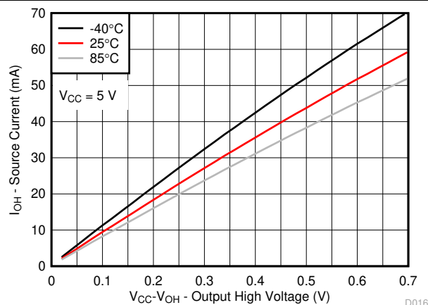
Figure 5-15. I/O Source Current vs Output High Voltage for Different Temperature ( T_A ) for V_{CC} = 5\text{V}
