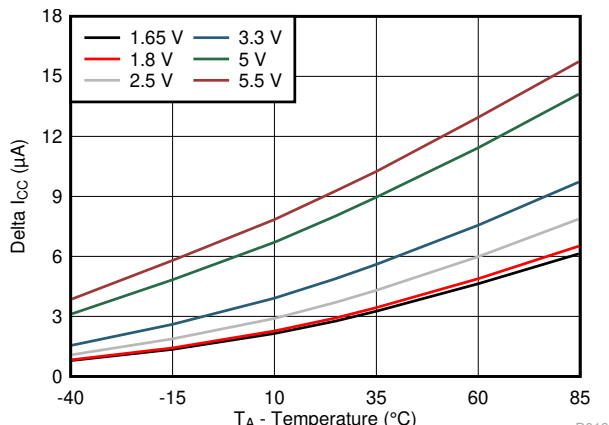
Figure 5-18. \Delta I_{CC} vs Temperature for Different V_{CC} ( V_I = V_{CC} - 0.6\text{V} )
