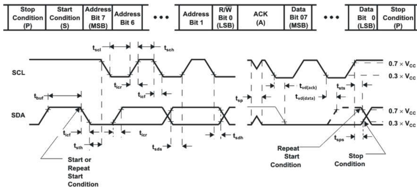
VOLTAGE WAVEFORMS
