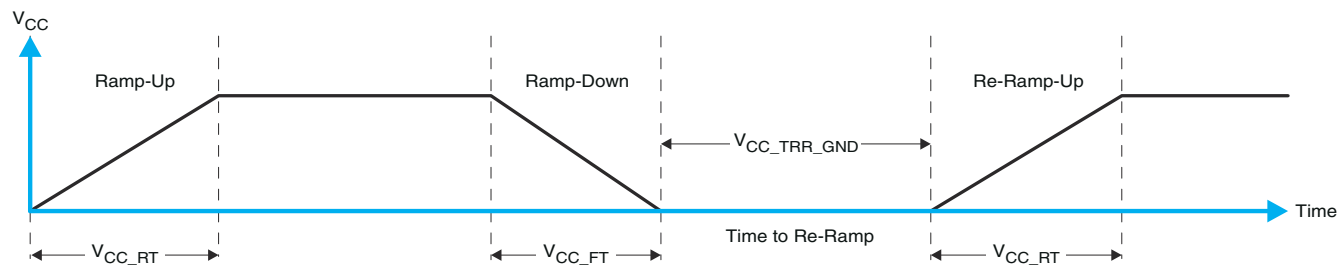
Figure 7-6. V_{CC} Is Lowered Below 0.2V Or 0V And Then Ramped Up To V_{CC}
