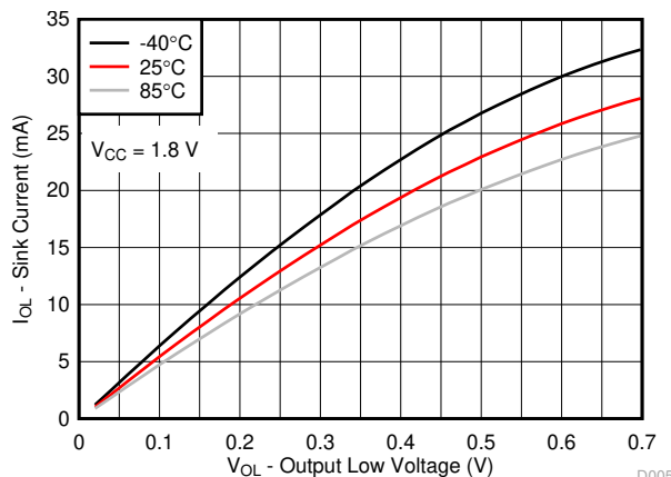
Figure 5-5. I/O Sink Current vs Output Low Voltage for Different Temperature ( T_A ) for V_{CC} = 1.8\text{V}
