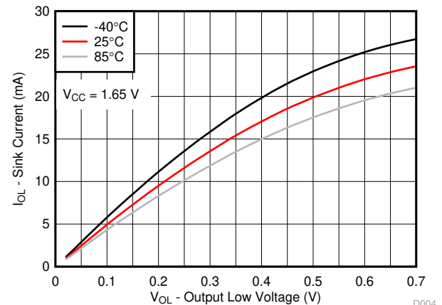
Figure 5-4. I/O Sink Current vs Output Low Voltage for Different Temperature ( T_A ) for V_{CC} = 1.65\text{V}
