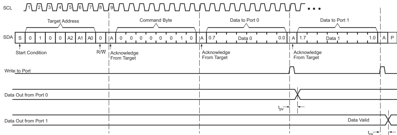
Figure 6-7. Write to Output Port Registers
