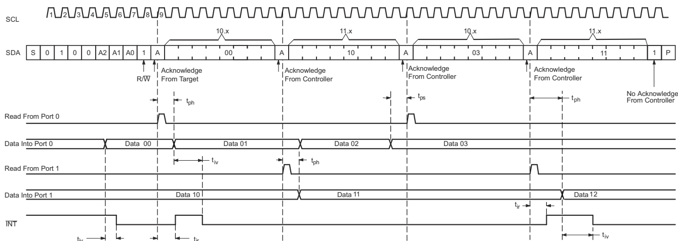
Figure 6-9. Read Input Port Register, Scenario 1
