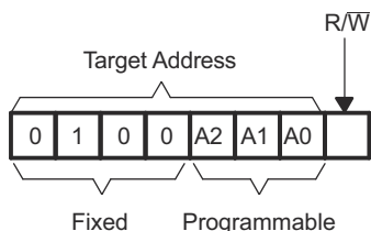
Figure 6-11. TCA9535 Address
