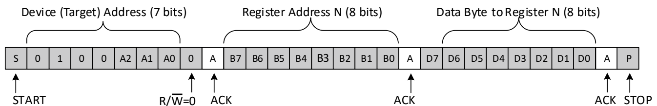
Figure 6-5. Write to Register
