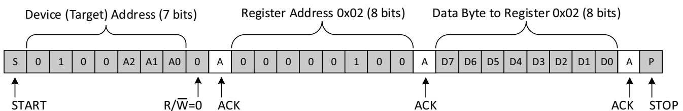
Figure 6-6. Write to the Polarity Inversion Register
