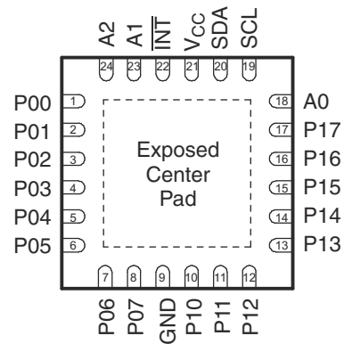
Figure 4-2. RTW (WQFN), RGE (VQFN) Package 24-Pin (Top View)
