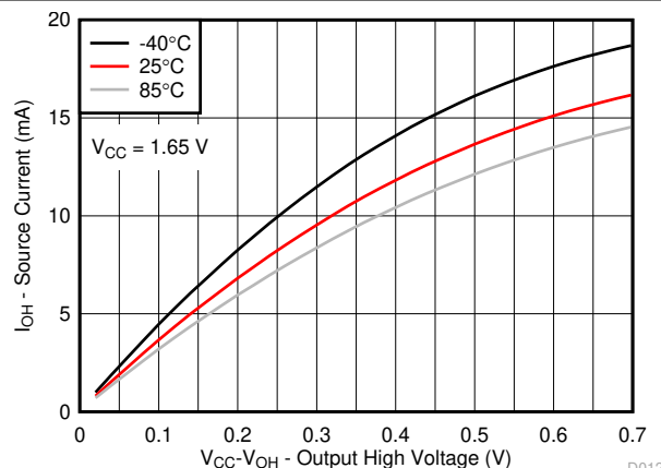
Figure 5-11. I/O Source Current vs Output High Voltage for Different Temperature ( T_A ) for V_{CC} = 1.65\text{V}
