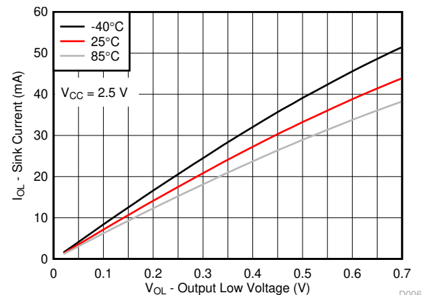
Figure 5-6. I/O Sink Current vs Output Low Voltage for Different Temperature ( T_A ) for V_{CC} = 2.5\text{V}
