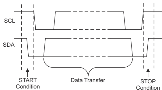
Figure 7-1. Definition of Start and Stop Conditions
