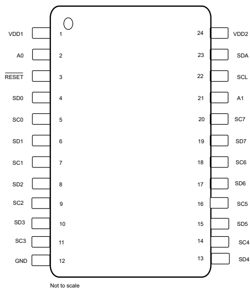
Figure 4-1. PW Package, 24-Pin TSSOP (Top View)
