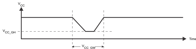
Figure 8-5. Glitch Width and Glitch Height
