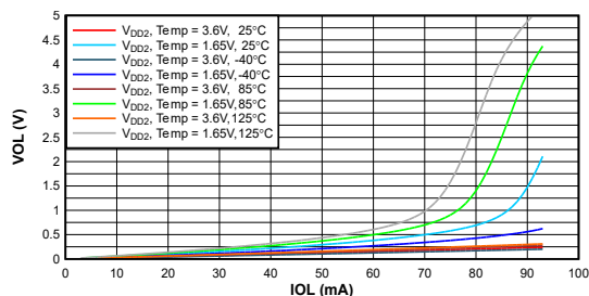
Figure 5-1. SDA Output Low Voltage ( V_{OL} ) vs Load Current ( I_{OL} ) at V_{DD2} Levels = 3.6V, 1.65V and T_A = -40 °C, 25 °C, 85 °C, 125 °C
