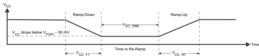
Figure 8-4. Power-On Reset Waveform
