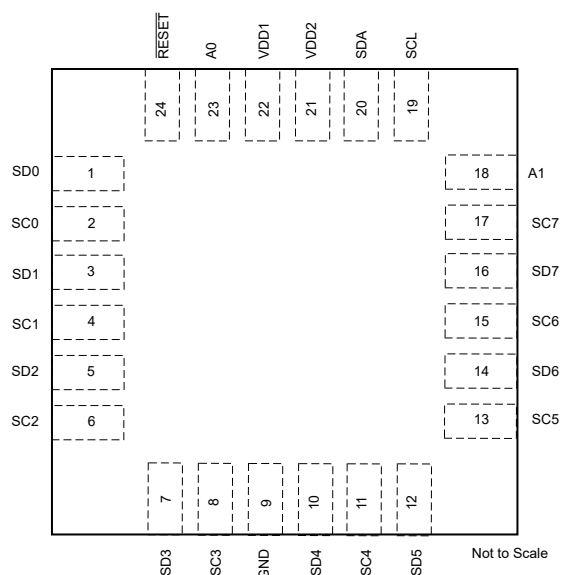
Figure 4-2. RGE Package, 24-Pin VQFN (Top View)
