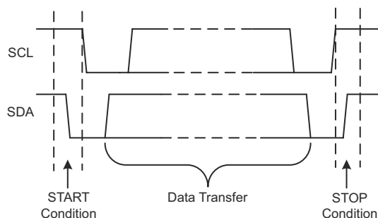
Figure 7-1. Definition of Start and Stop Conditions
