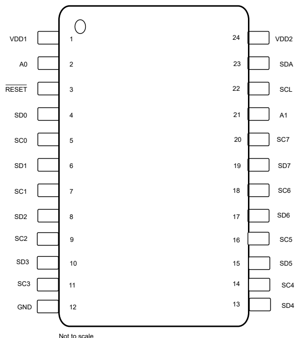
Figure 4-1. PW Package, 24-Pin TSSOP (Top View)
