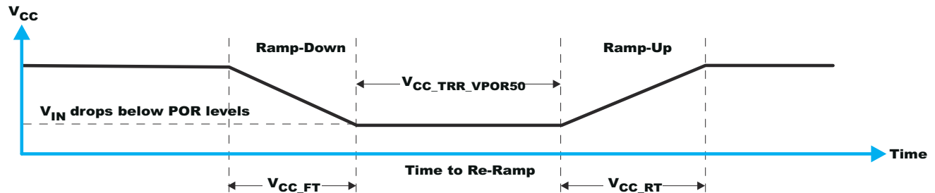
Figure 8-7. V is lowered below the POR threshold, then ramped back up
