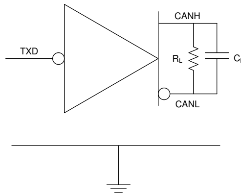
Figure 5. I_{CC} Test Circuit
