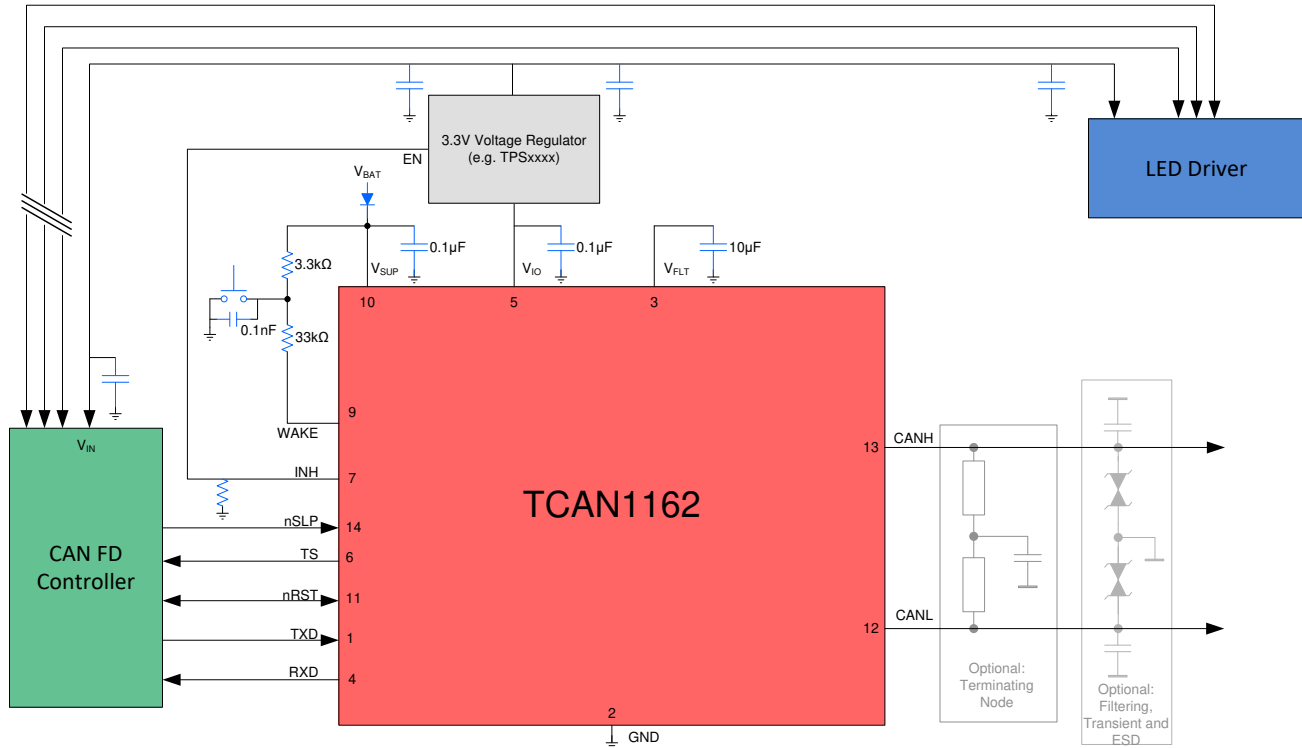
Simplified Schematic
