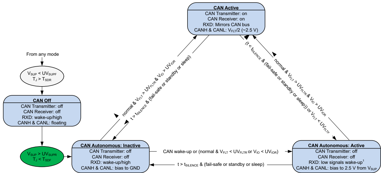
Figure 7-8. TCAN1162 CAN Transceiver State Machine
