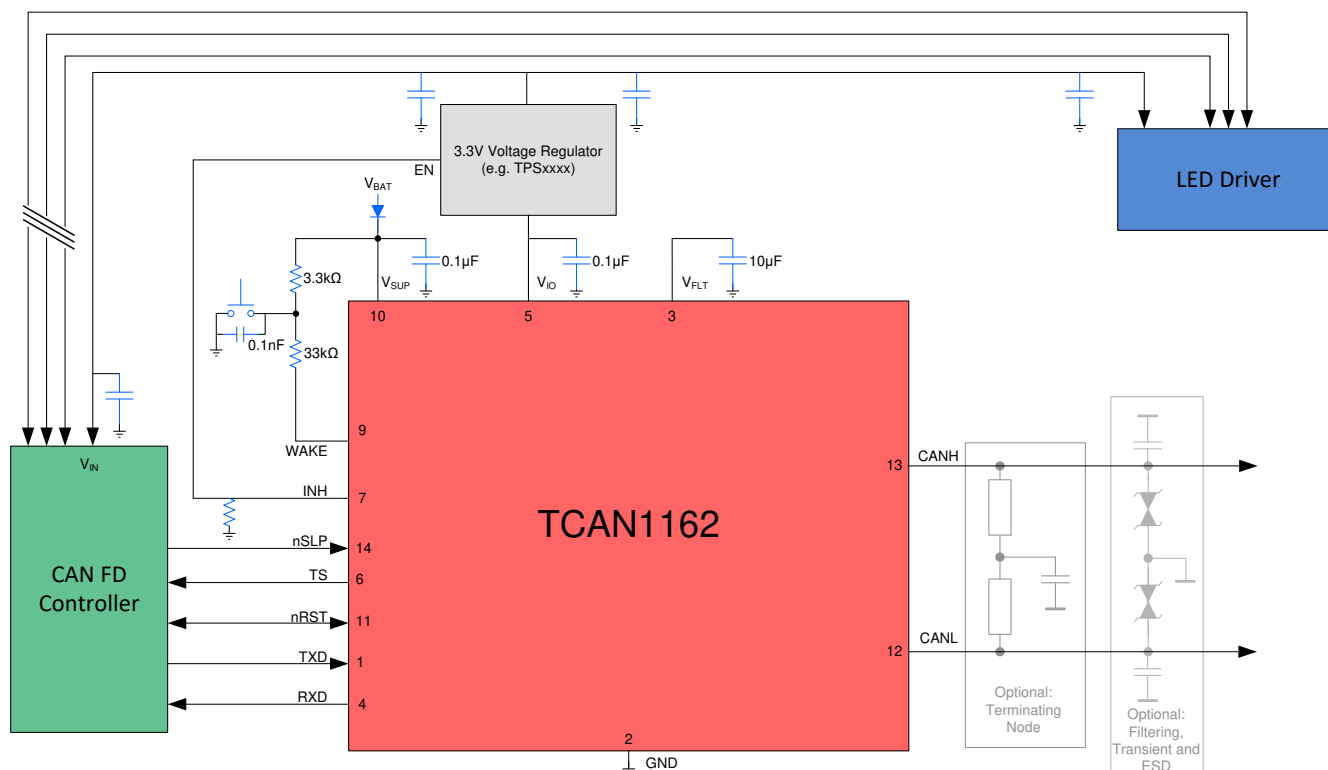
Figure 8-1. Typical Application
