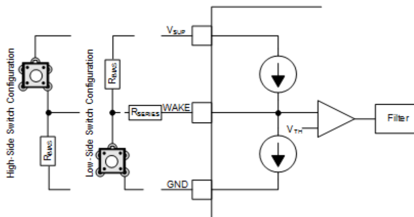
Figure 7-15. WAKE Circuit Example
