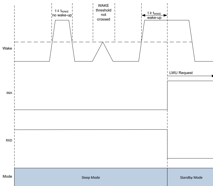
Figure 7-16. LWU Request Rising Edge
