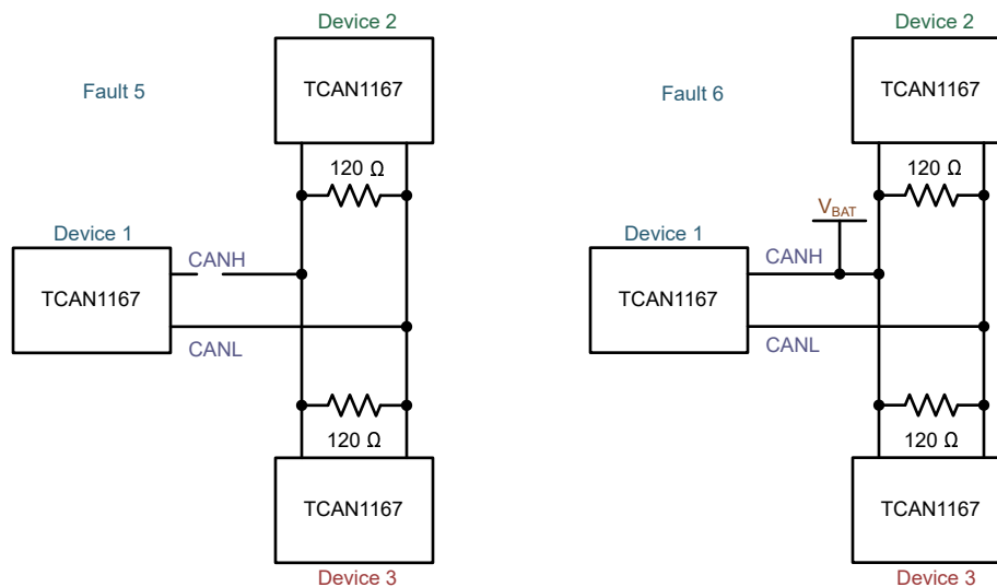
Figure 7-10. Fault 5 and 6 Examples
