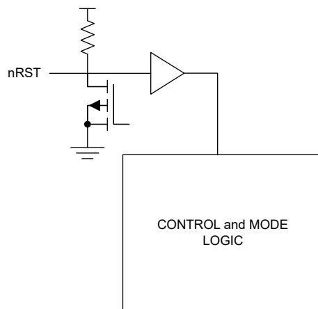
Figure 7-1. nRST Circuit
