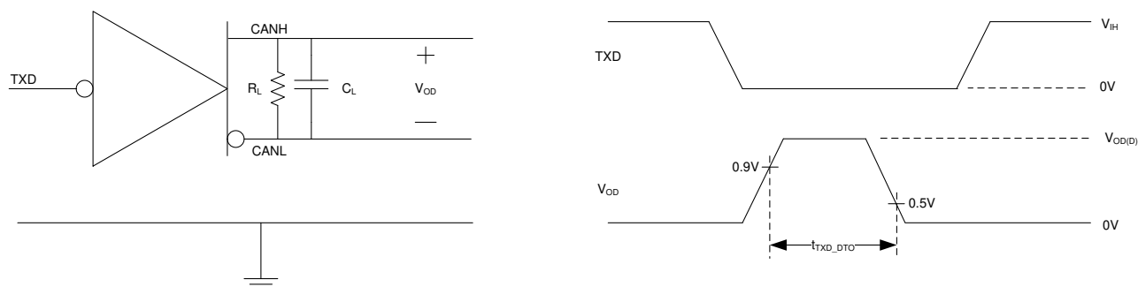
Figure 6-7. TXD Dominant Timeout Test Circuit and Measurement
