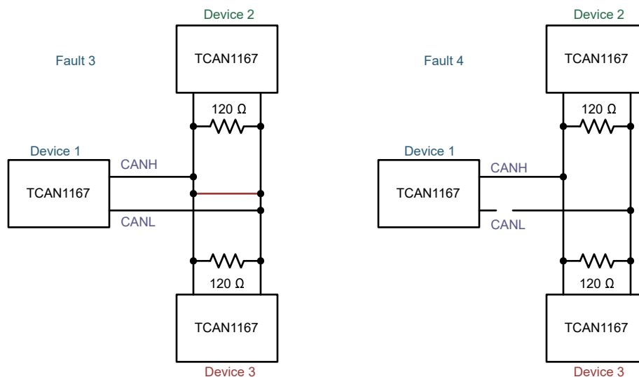
Figure 7-9. Fault 3 and 4 Examples
