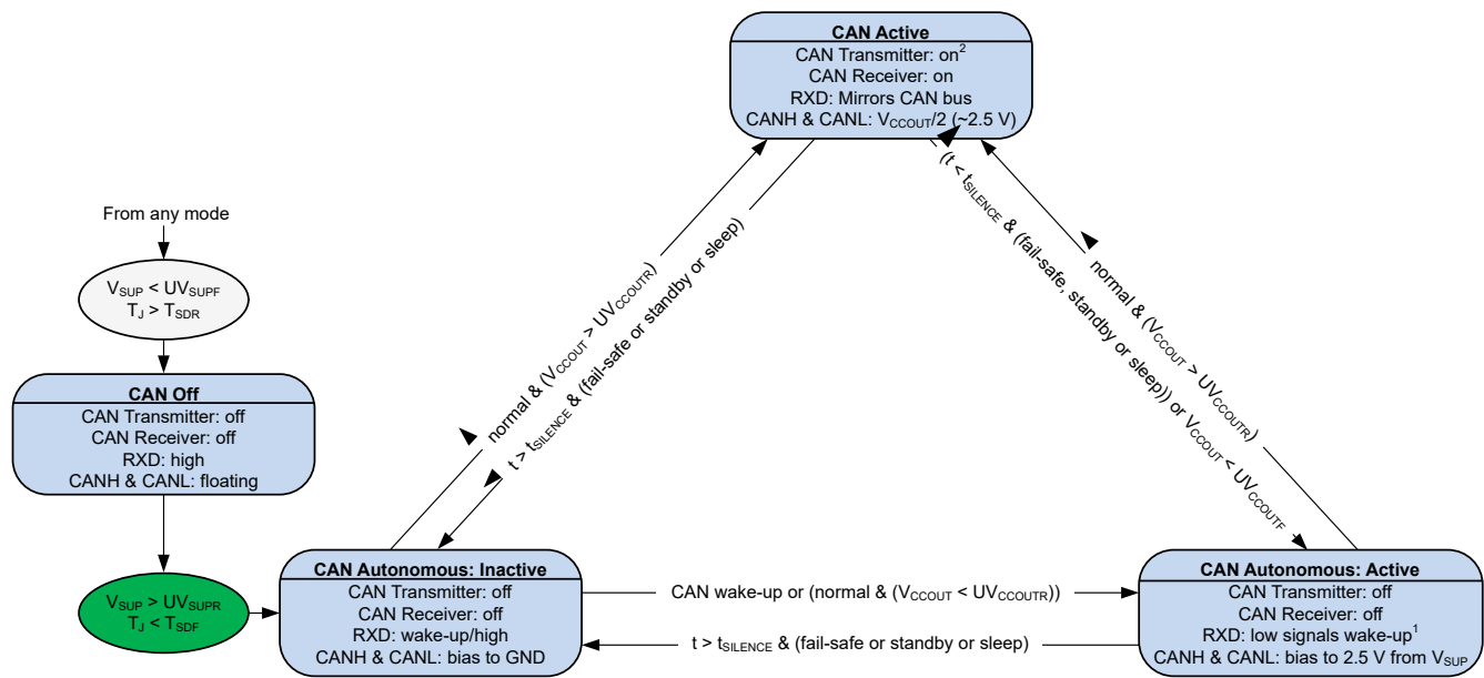
Figure 7-18. TCAN1167 CAN Transceiver State Machine
