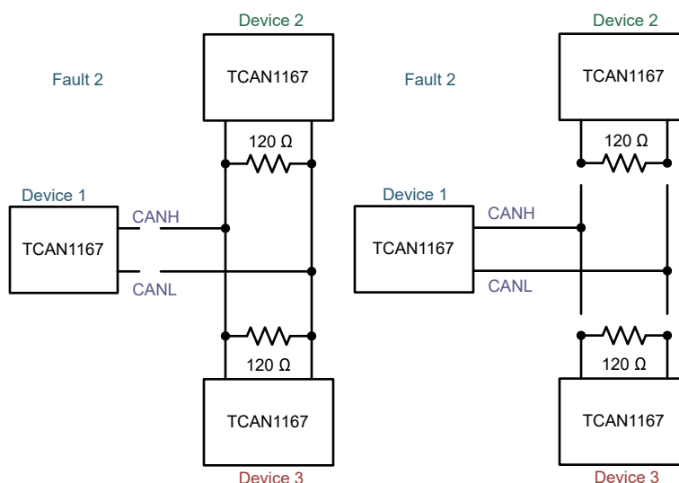
Figure 7-8. Fault 2 Examples
