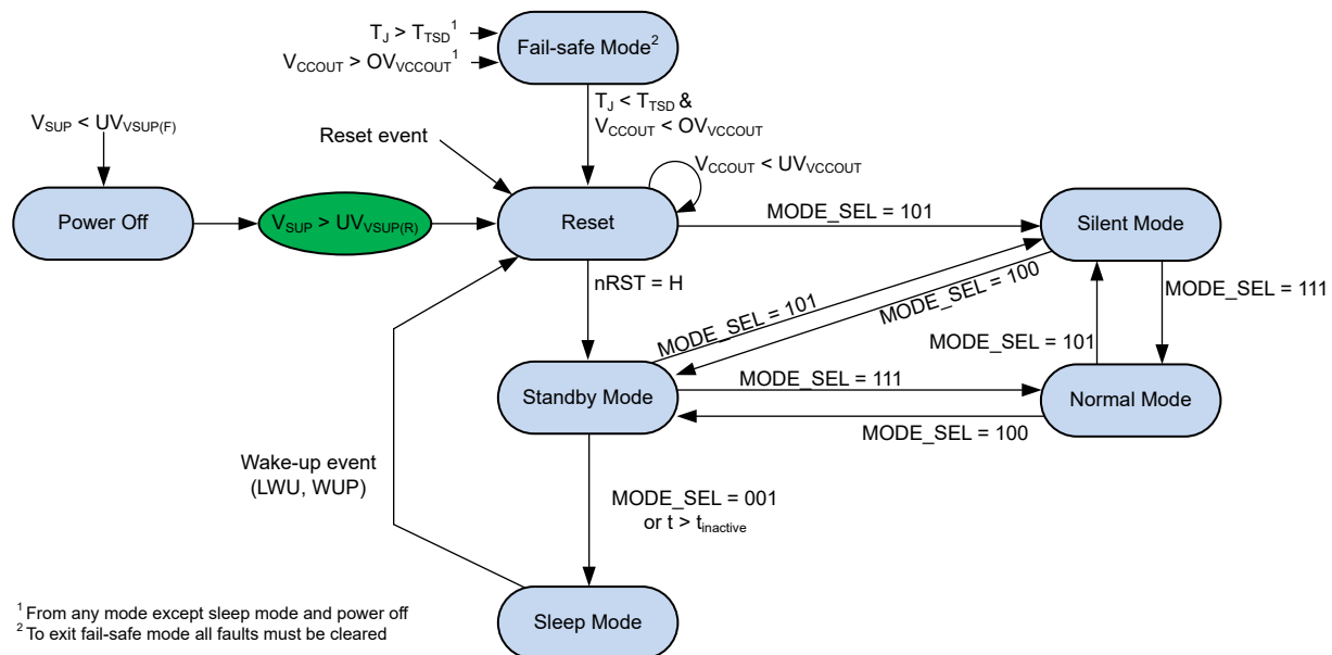
Figure 7-13. TCAN1167 State Machine
