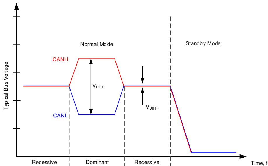
Figure 7-19. Bus States
