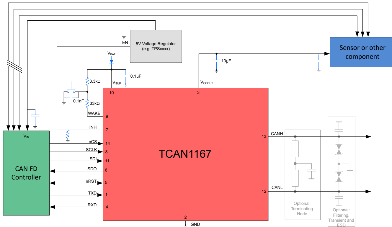
Figure 8-1. Typical Application
