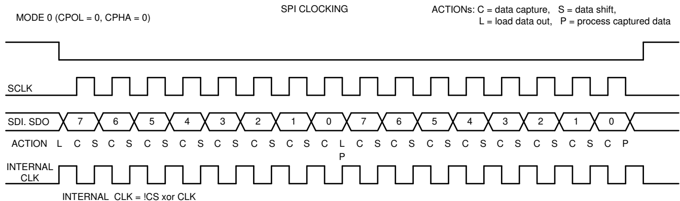
Figure 7-20. SPI Clocking
