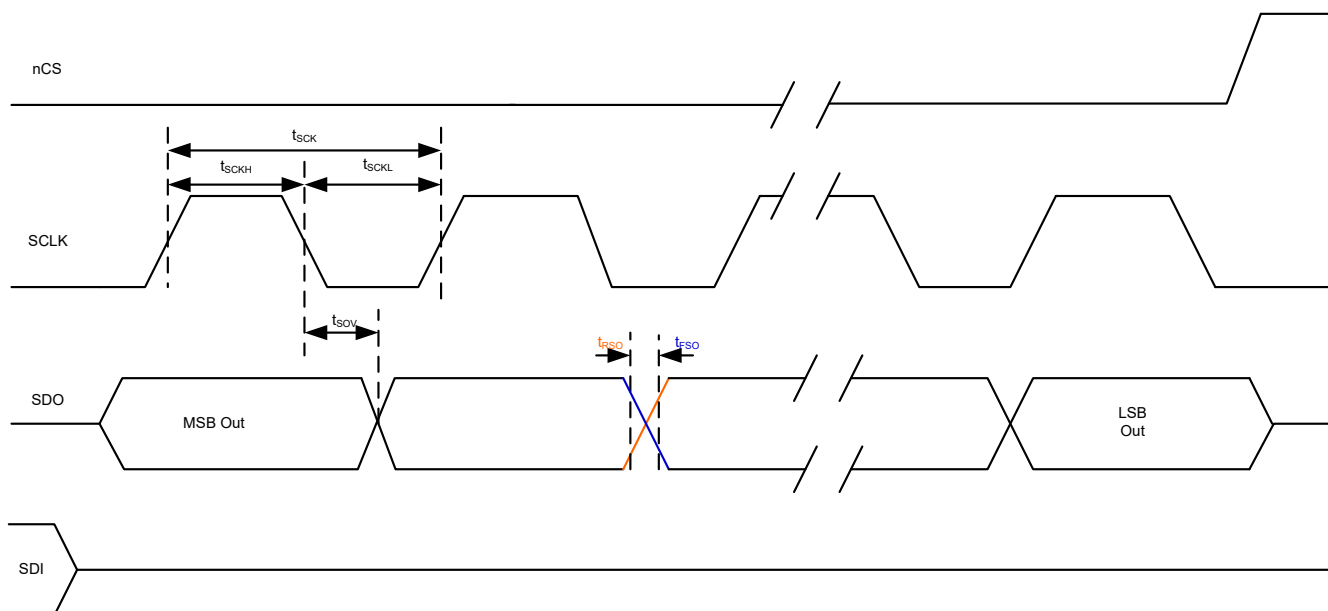
Figure 6-13. SPI AC Characteristic Read
