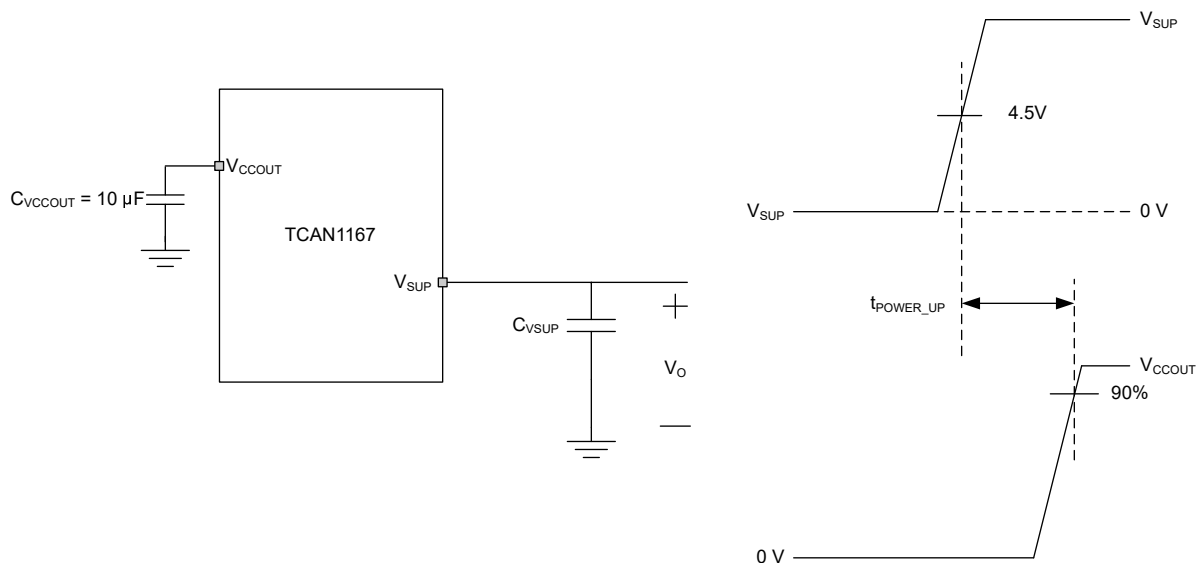
Figure 6-9. t_{POWER\_UP} Timing Measurement
