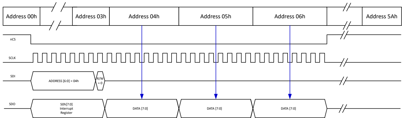
Figure 7-24. 32-bit SPI Burst Read
