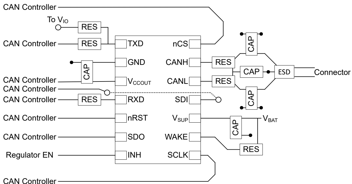
Figure 8-4. TCAN1167 Example Layout
