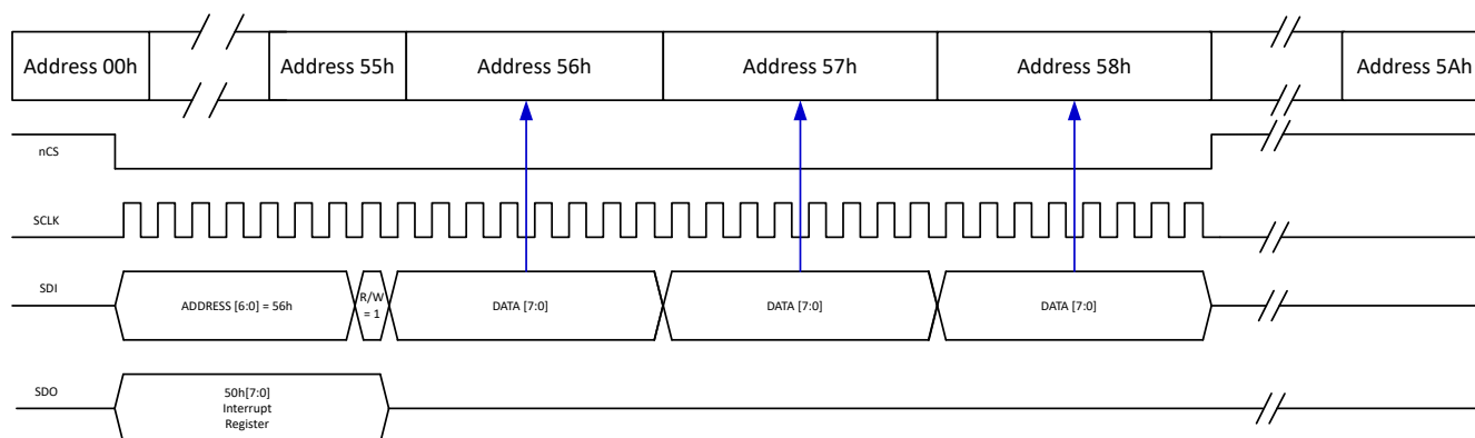
Figure 7-22. 32-bit SPI Burst Write
