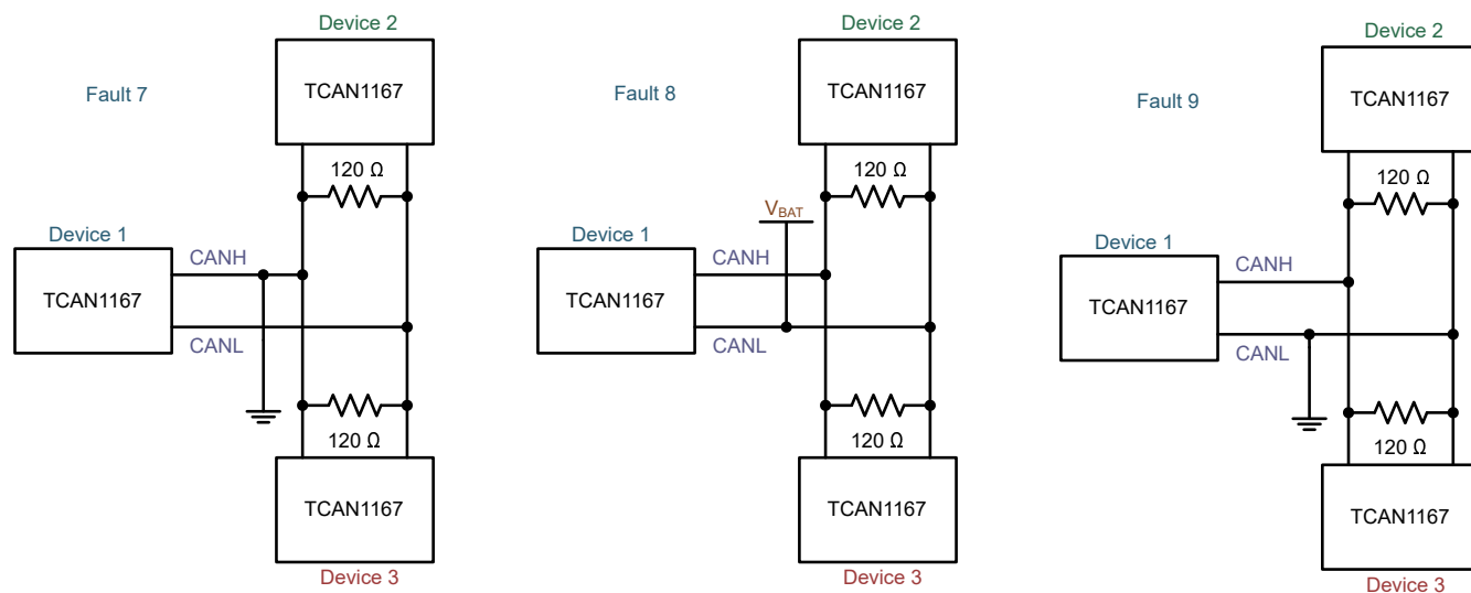
Figure 7-11. Fault 7, 8 and 9 Examples
