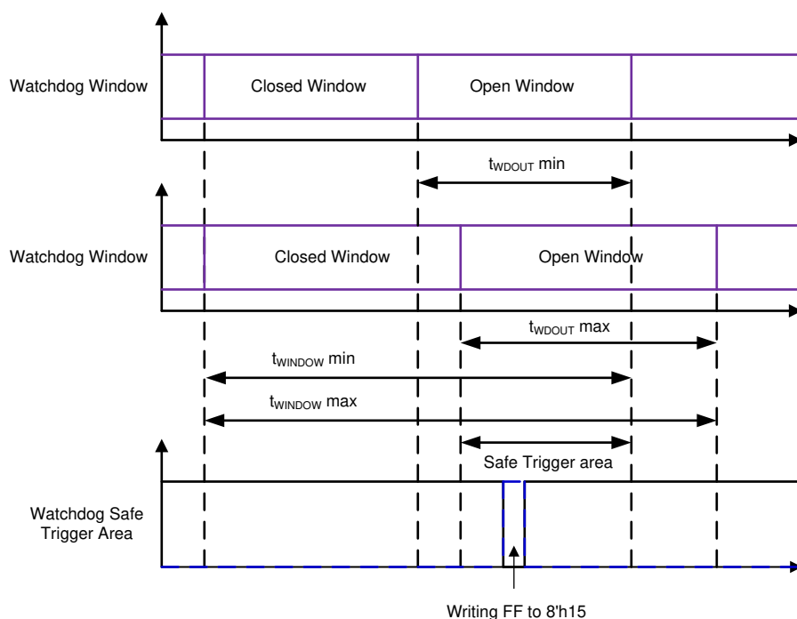
Figure 7-3. Window Watchdog Timing Diagram
