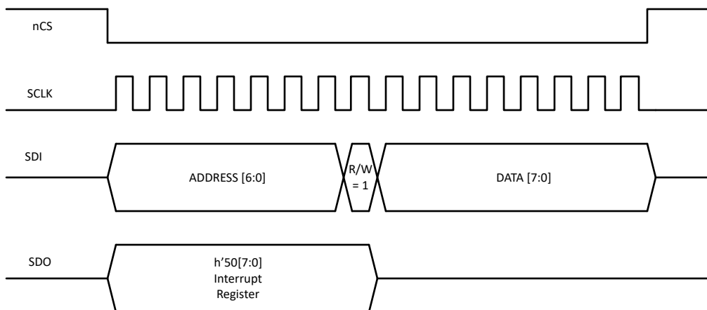
Figure 7-21. SPI Write
