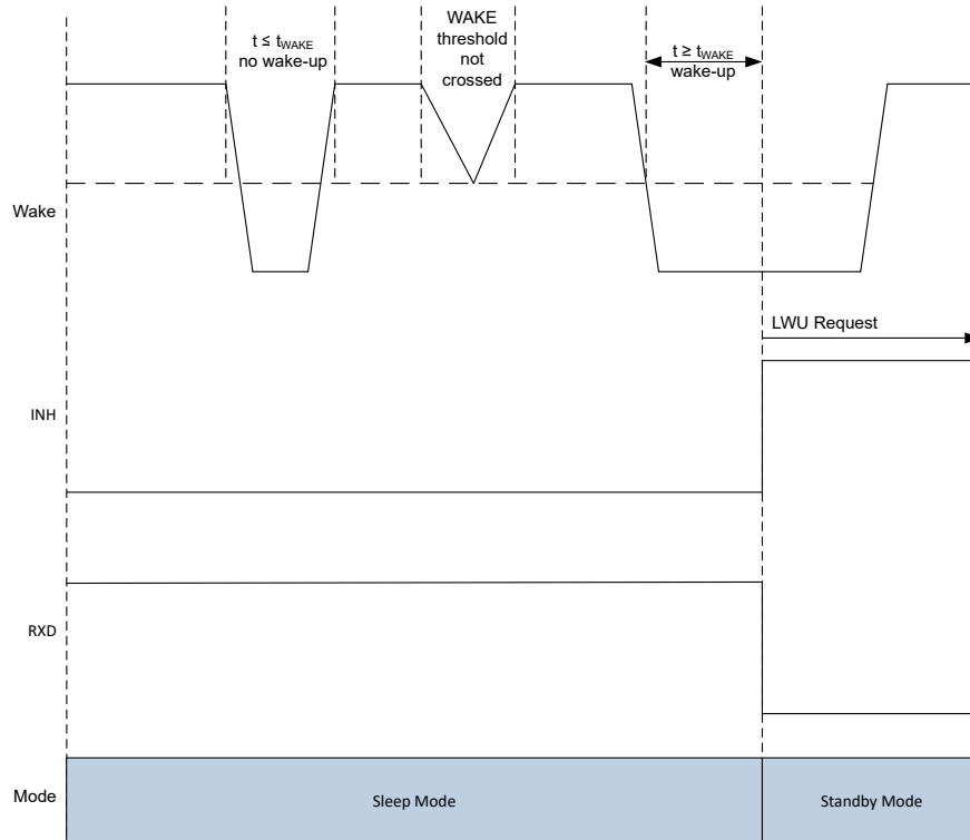
Figure 7-17. LWU Request Falling Edge
