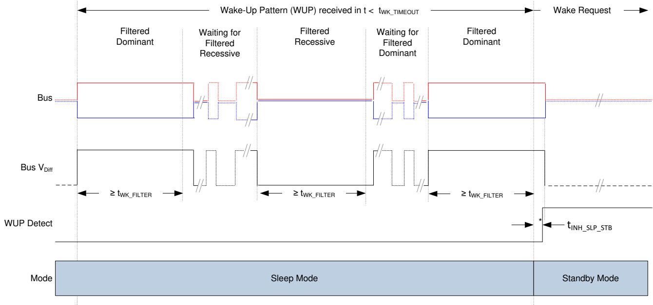
Figure 7-14. Wake-Up Pattern (WUP) From Sleep Mode To Standby Mode
