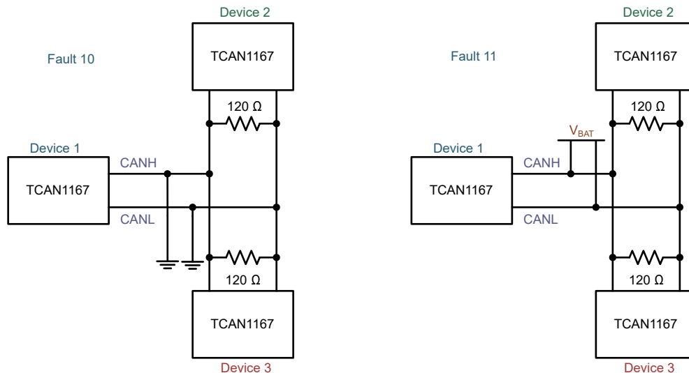
Figure 7-12. Fault 10 and 11 Examples
