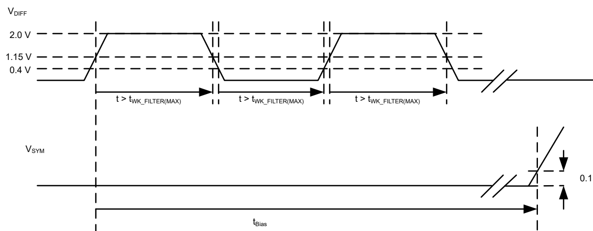
Figure 6-11. Test Signal Definition for Bias Reaction Time Measurement
