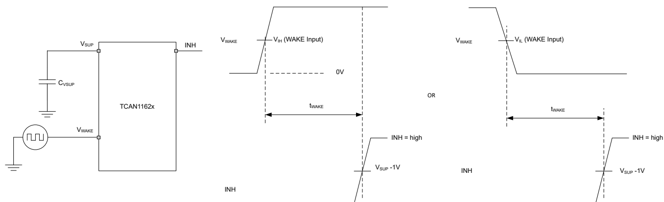
Figure 6-10. t_{WAKE} While Monitoring INH Output
