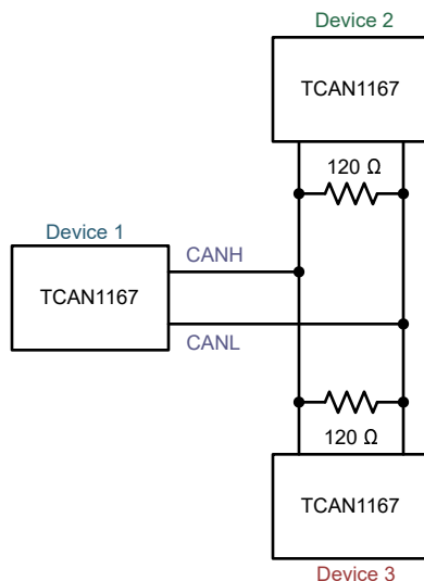
Figure 7-7. Three Node Example
