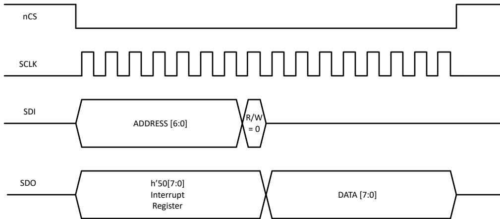
Figure 7-23. SPI Read
