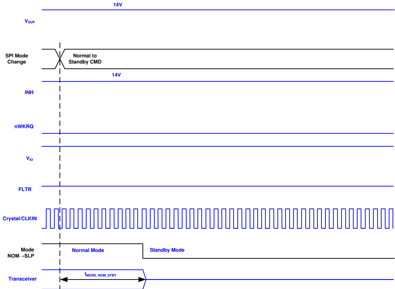
Figure 17. Normal to Standby Timing
