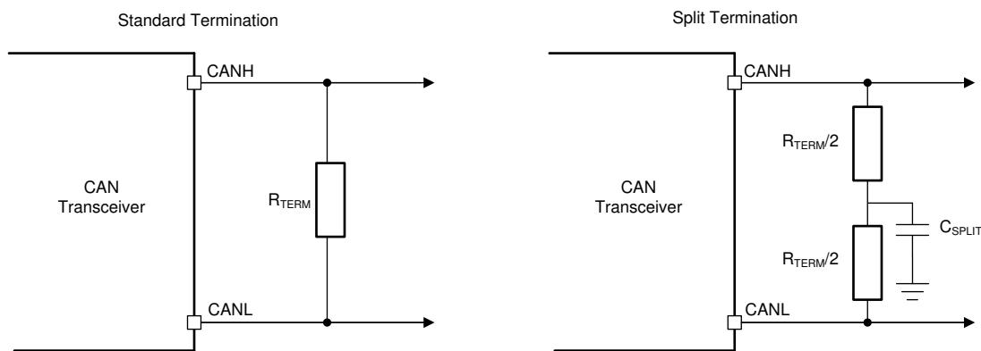
Figure 102. CAN Bus Termination Concepts
