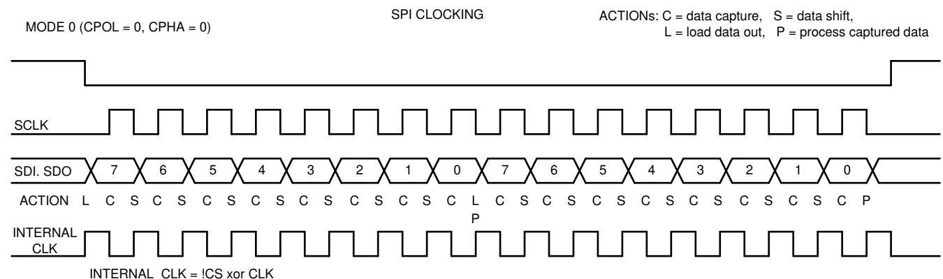
Figure 33. SPI Clocking
