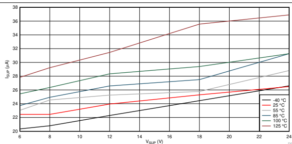
Figure 1. I_{\text{SUP}} VS V_{\text{SUP}} Sleep Mode
