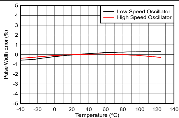
Figure 5-2. Pulse Width Error vs Temperature
