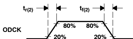
Figure 1. Rise and Fall Time of ODClock
