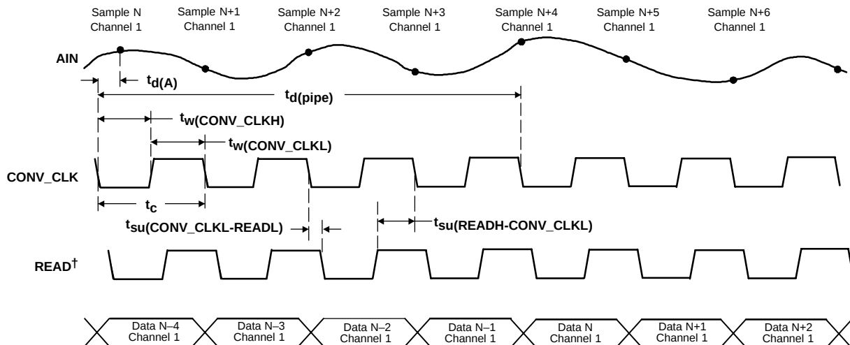
Figure 25. Conversion Timing in 1-Channel Operation
