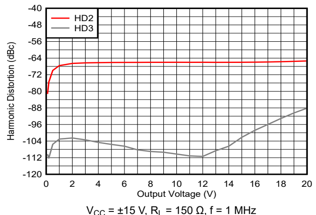
Figure 5-18. Harmonic Distortion vs Peak-to-Peak Output Voltage
