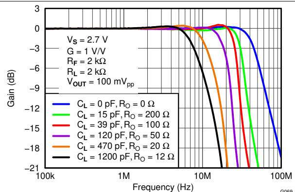
Figure 78. Frequency Response for Various R_O and C_L Values
