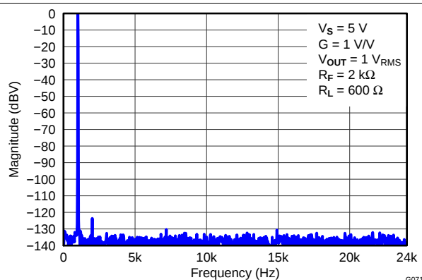
Figure 83. 1-kHz FFT Plot on Audio Analyzer
