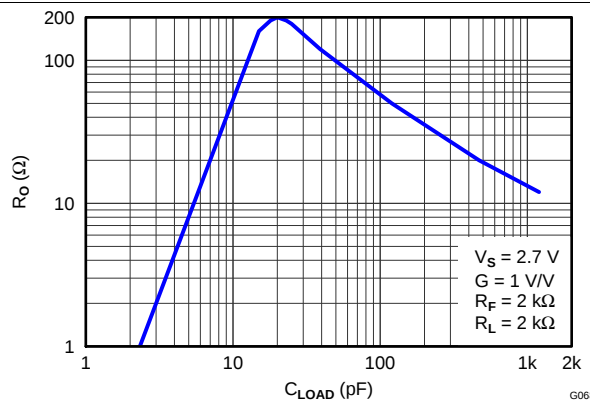
Figure 79. Recommended Series Output Resistor vs Capacitive Load for Flat Frequency Response
