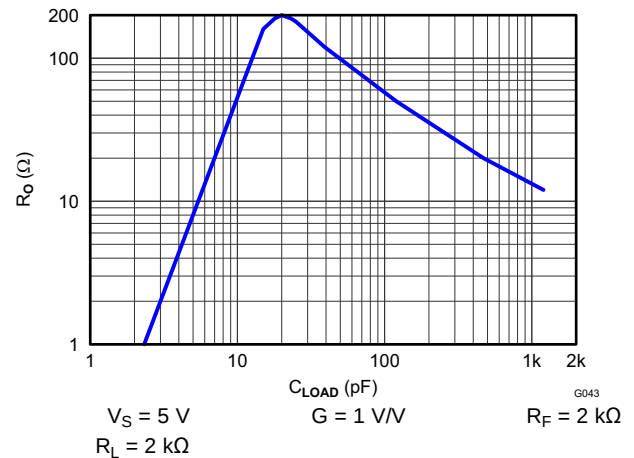
Figure 52. R_O vs C_{LOAD}
