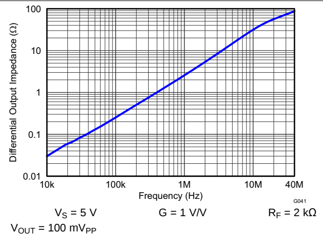
Figure 50. Main Amplifier Differential Output Impedance vs Frequency
