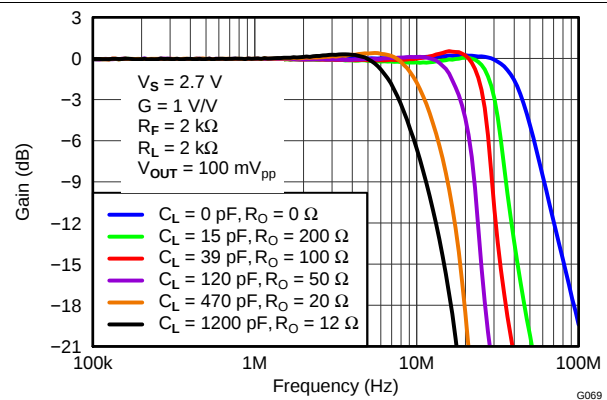
Figure 80. Frequency Response for Various R_O and C_L Values
