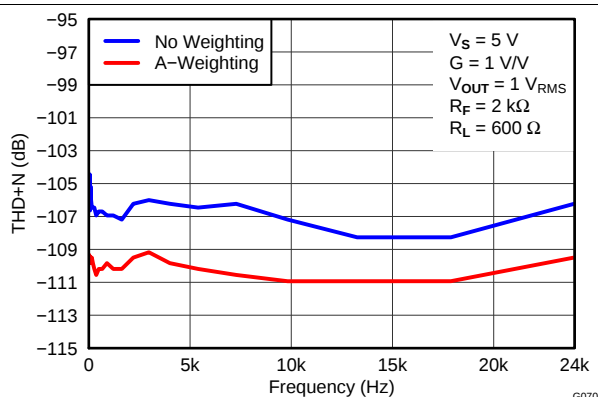
Figure 82. THD+N on Audio Analyzer, 10 Hz to 24 kHz
